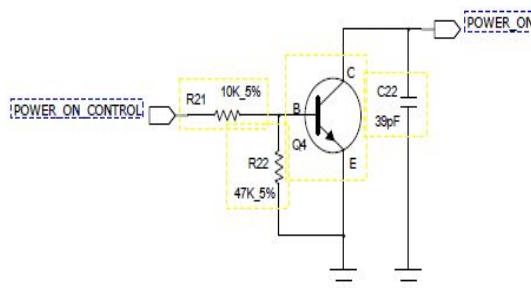
Figure 5-3 POWER_ON Reference Design
