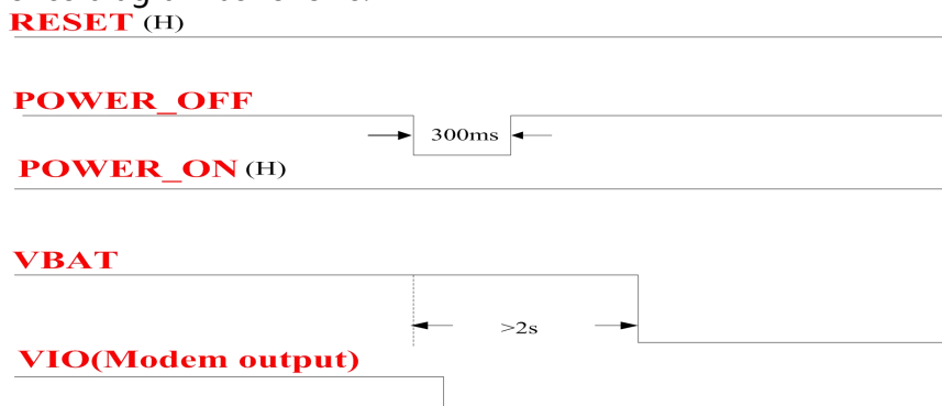
Figure 5-4 Power off Timing Control Diagram
