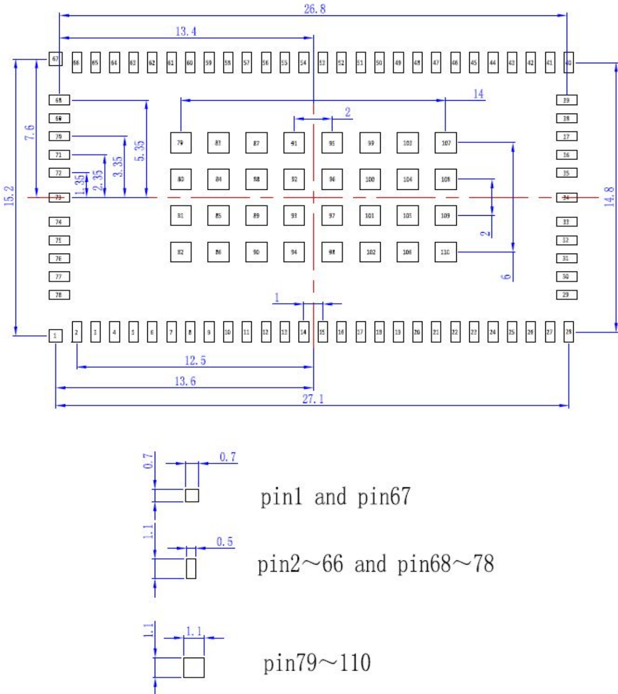
Figure 3- 2 Recommended PCB Layout
