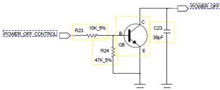
Figure 5-5 Recommended Design of POWER_OFF# Signal
