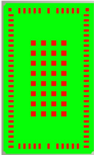
Figure 2- 2 Bottom View
