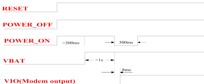
Figure 5-2 Timing Control
