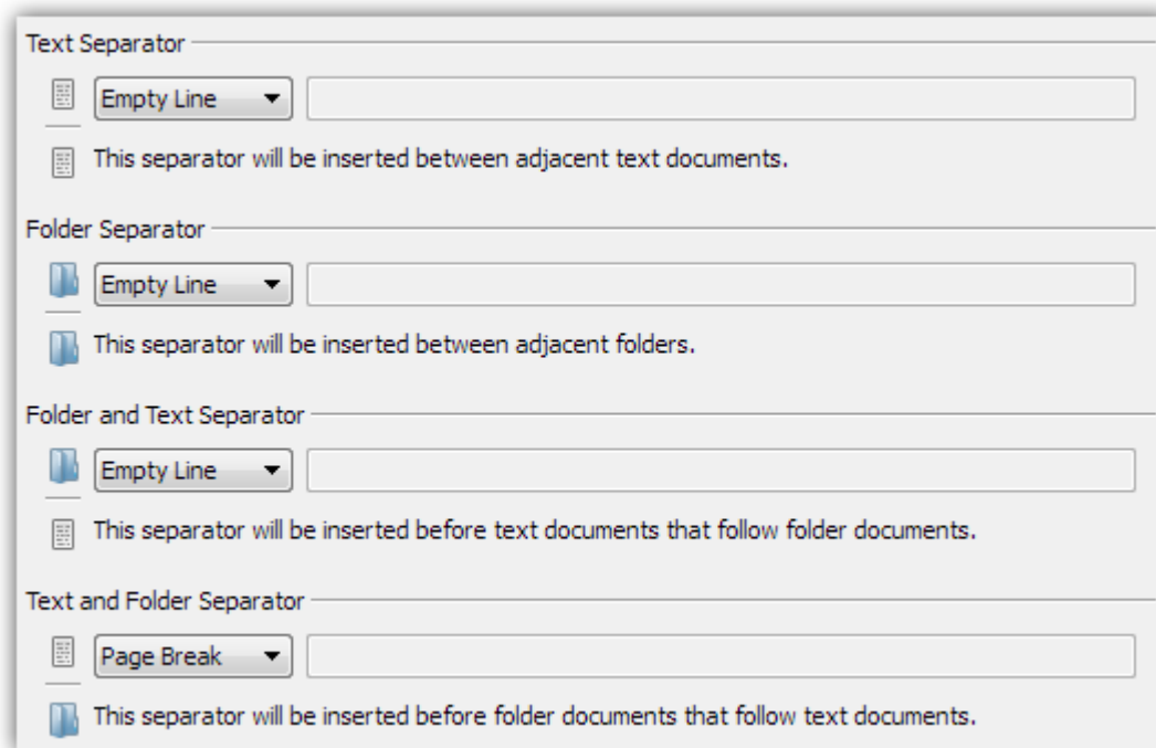
Figure 23.2: Compile—Separators Pane
