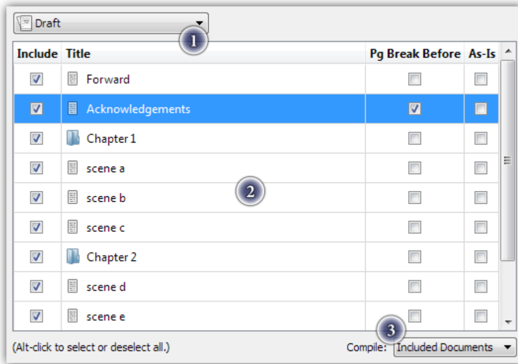
Figure 23.1: Compile—Contents Pane
