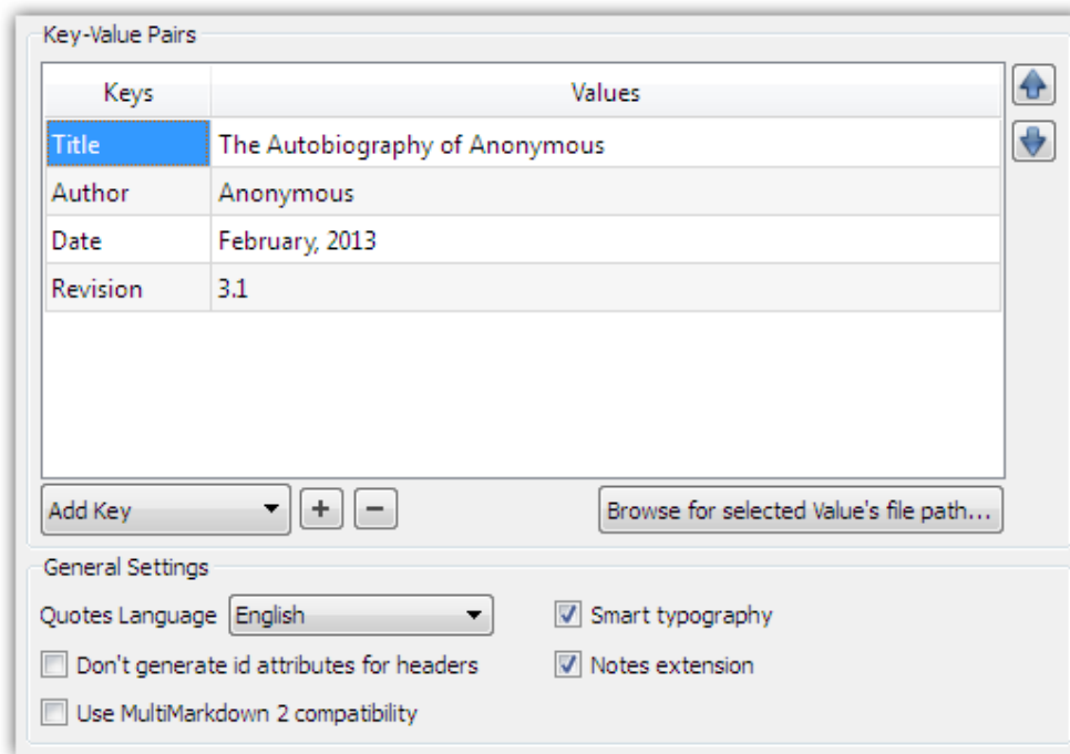
Figure 23.12: Compile—Meta-Data (MMD)
