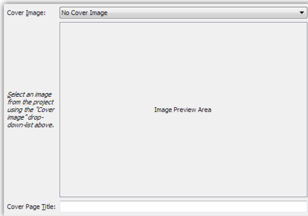
Figure 23.3: Compile—Cover & ToC
