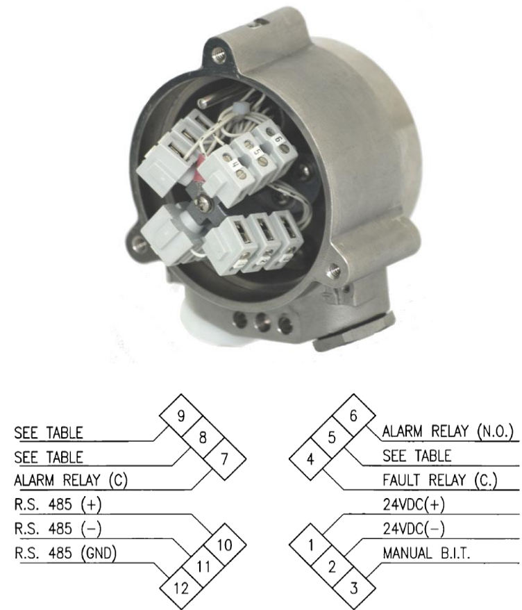
Figure 9: Wiring Terminals
