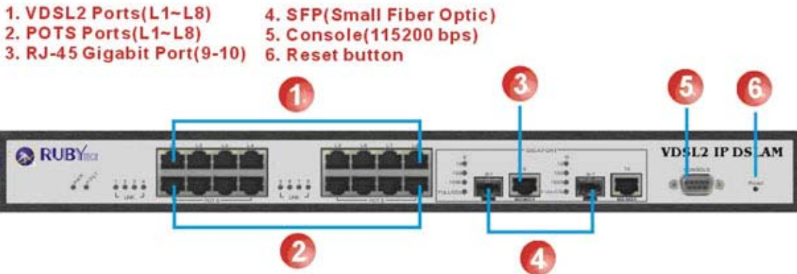
Figure Chapter 2.1 Front Panel description
