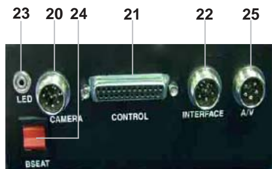
Figure 11 : Description of Rear Panel Control Head
