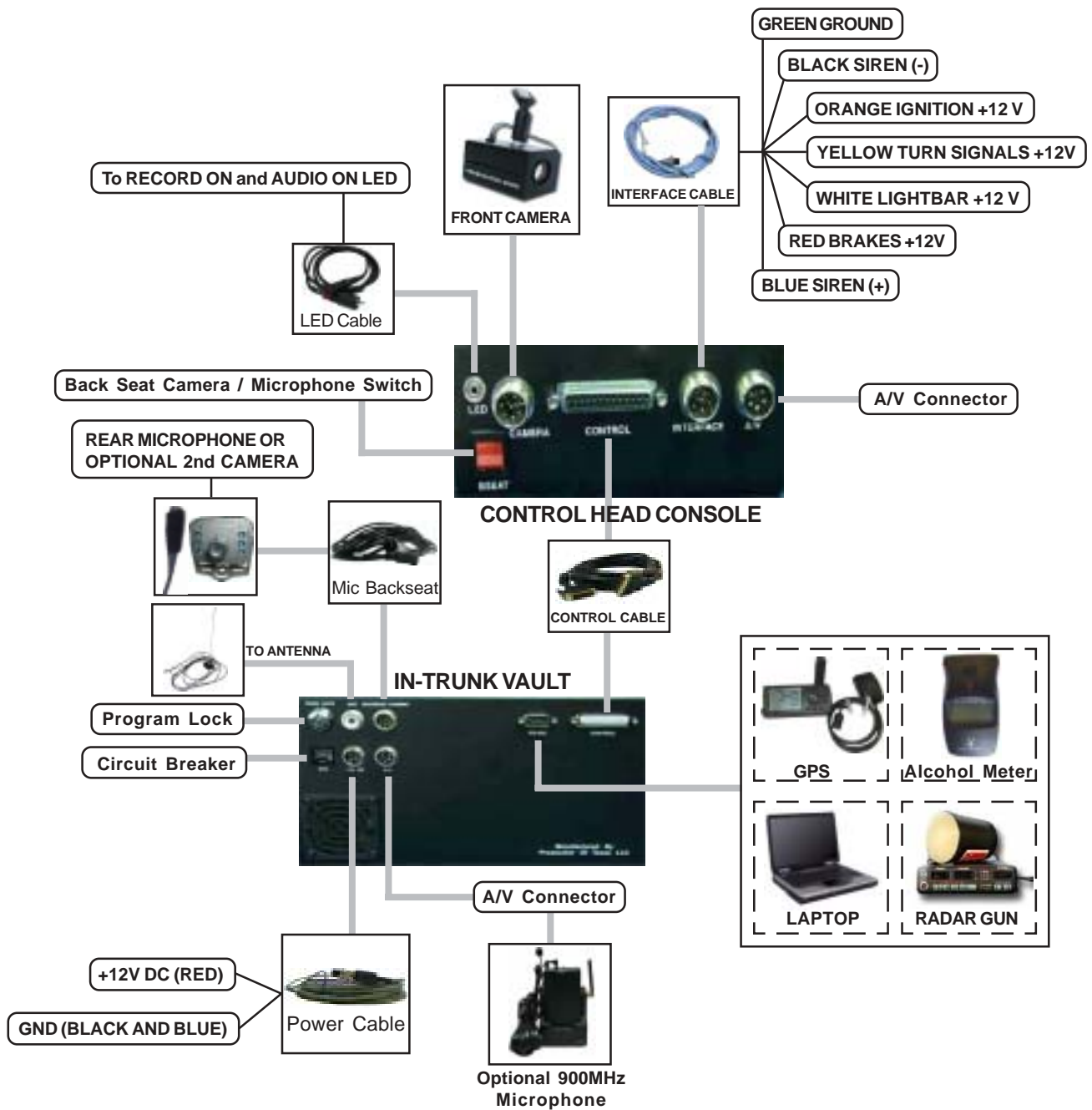
Figure 14 : Description of Connections
