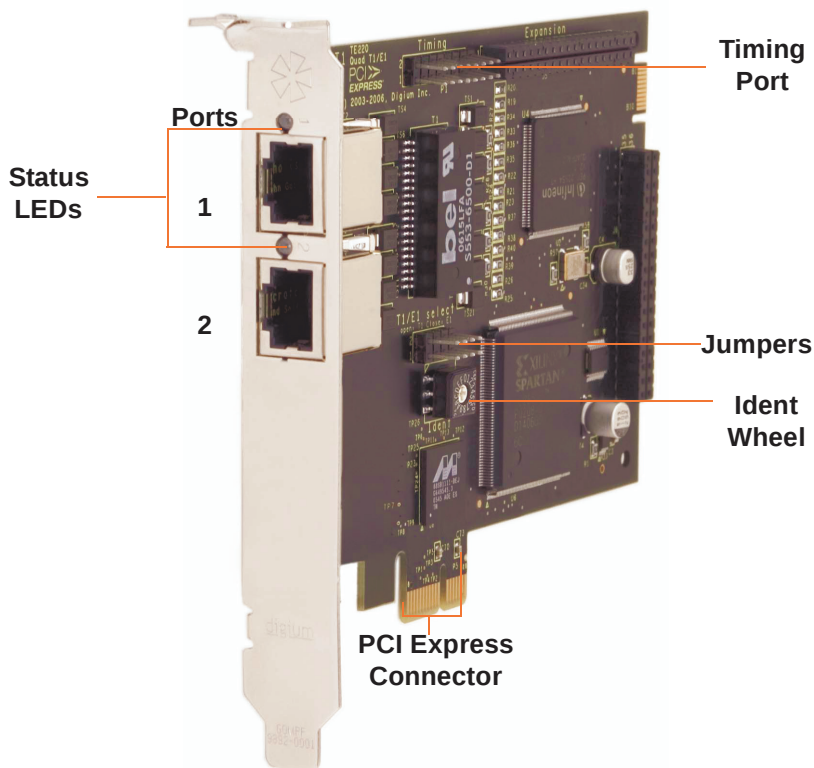
Figure 5: TE220 Card
