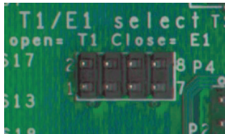
Figure 6: T1/E1 Jumpers
