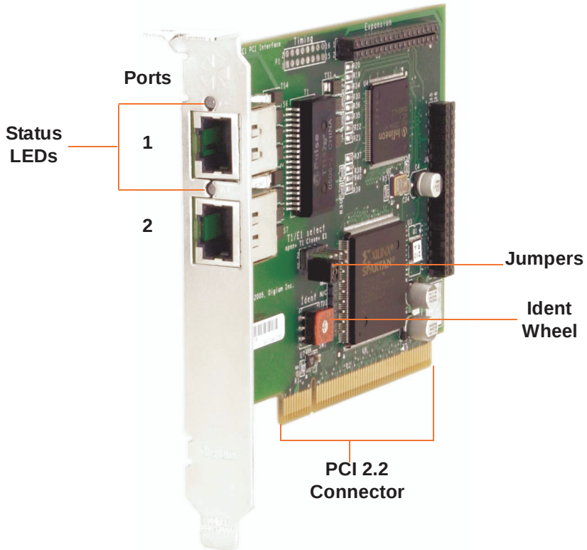
Figure 4: TE210P Card
