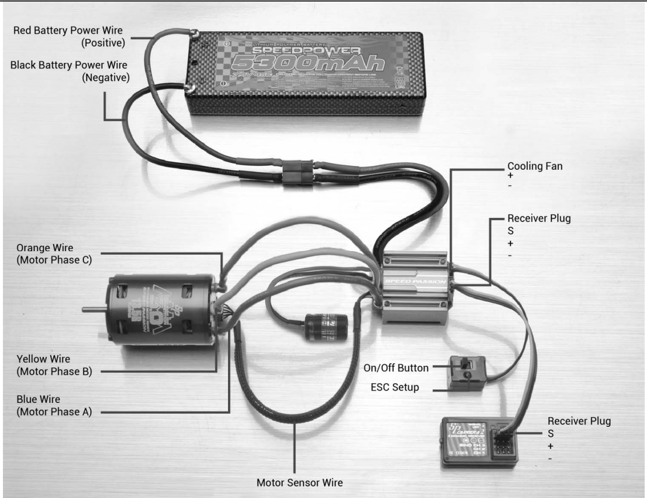
Picture A: Wiring with a brushless motor
