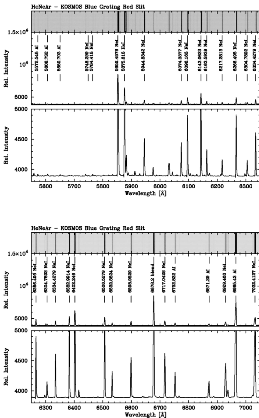
Figure 28: He-Ne-Ar spectra for blue VPH grism, red-offset slit.
