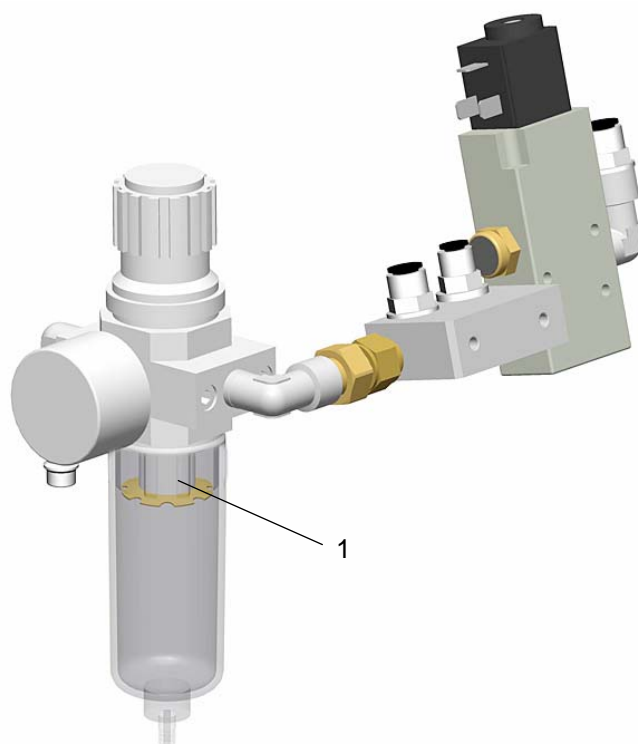
OptiFlex 2 S - Pneumatic group
