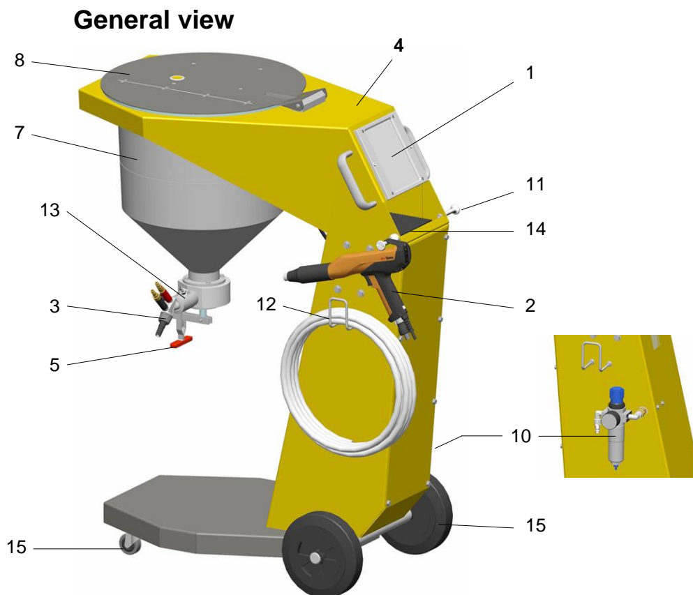
OptiFlex 2 S manual coating equipment - Structure
