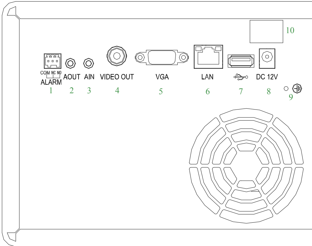
Rear panel of the NV0402S
