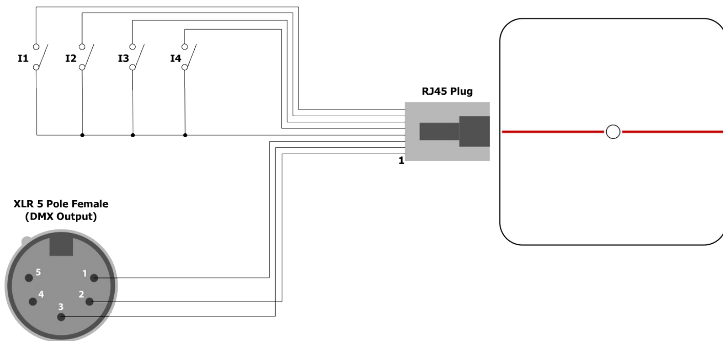
RJ45 Plug wiring example
