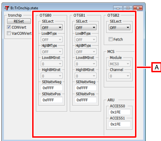
A OTGM/OTGB trace configuration for GTM
