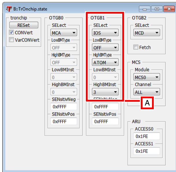
A Enable signal trace (IOS) for ATOM 3 on OTGB1.
