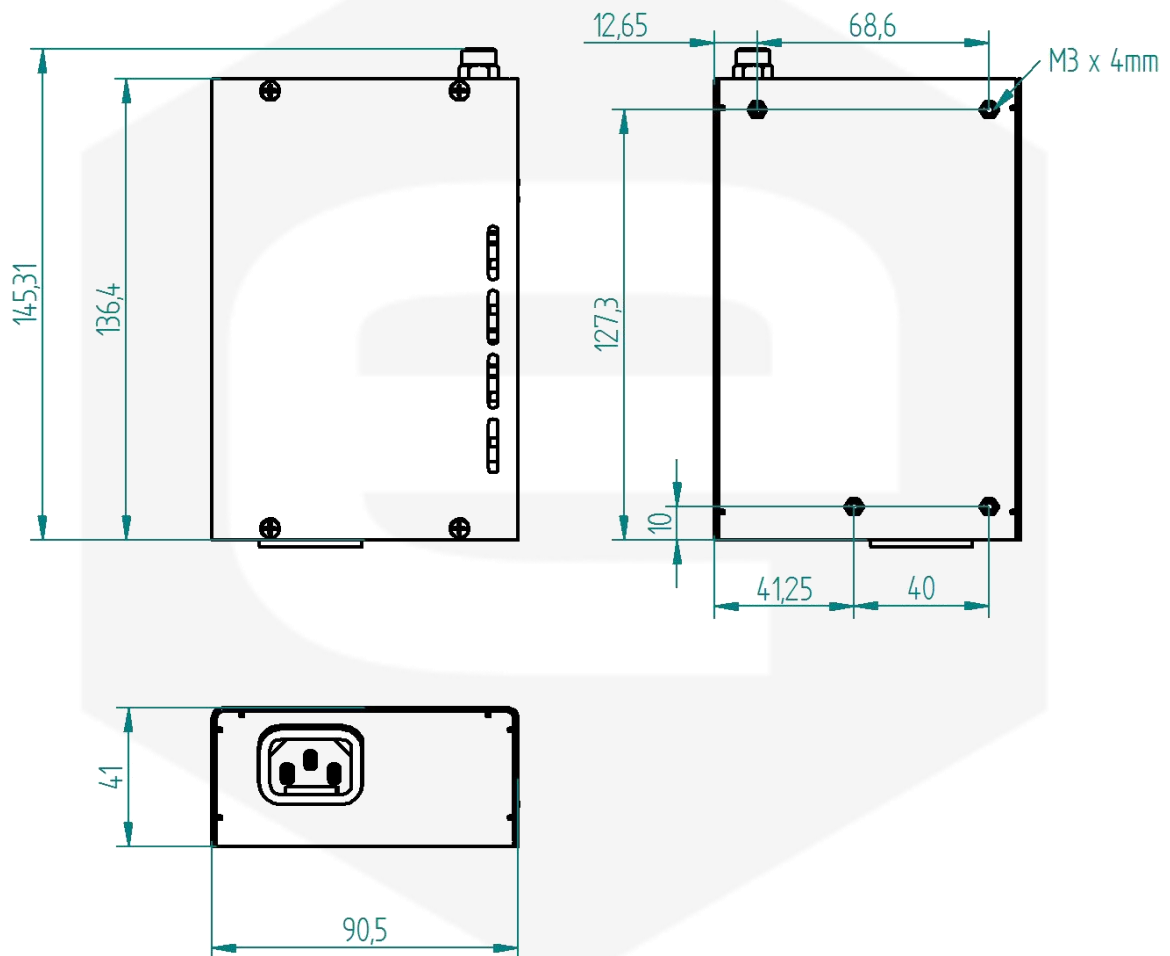
Figure 12: Mechanical drawings
