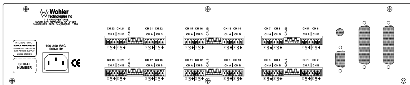
LM53-24 Rear Panel (Twenty Four-Channel with "Mini" Phoenix Connectors)
