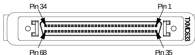
Figure 10-1 : Front Panel I/O Connector Numbering
