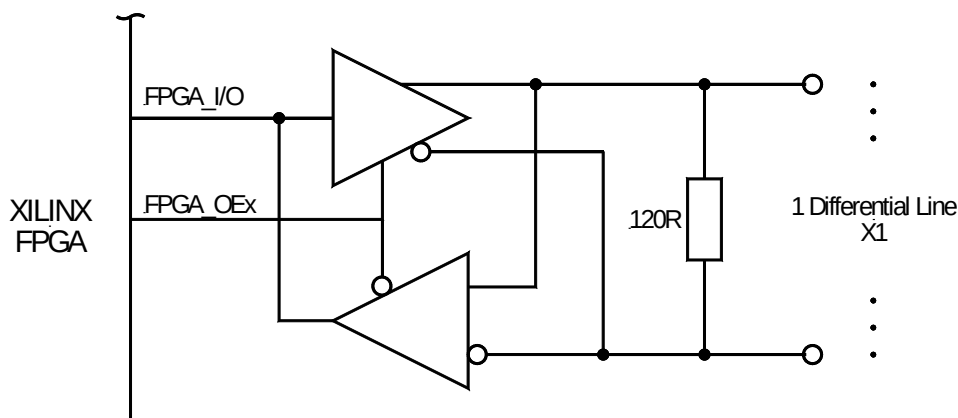
Figure 9-2 : Differential I/O Interface
