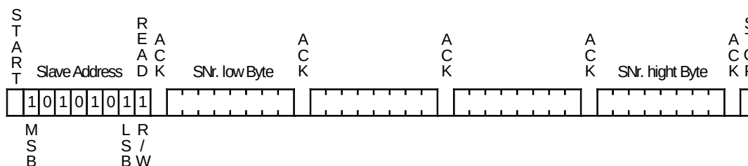
Figure 7-9 : Configuration FPGA Slave Access
