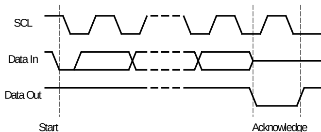
Figure 7-8 : Configuration FPGA Output Acknowledge
