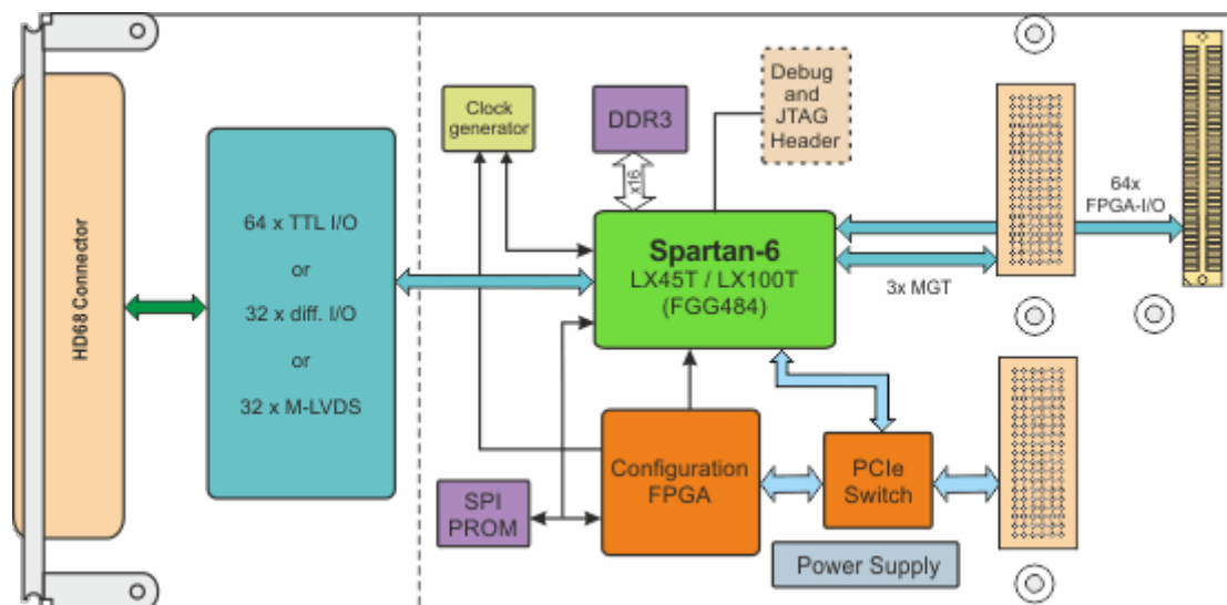
Figure 1-1 : Block Diagram
