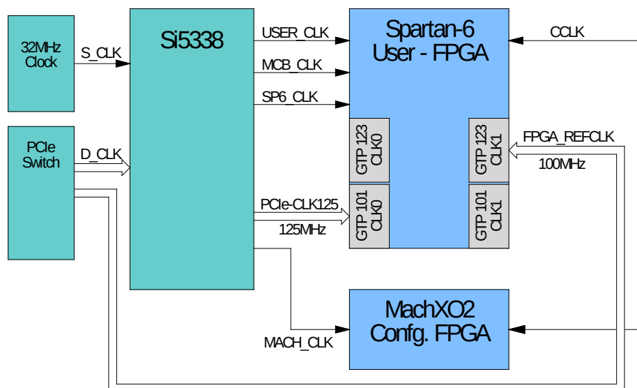
Figure 7-5 : FPGA Clock Sources
