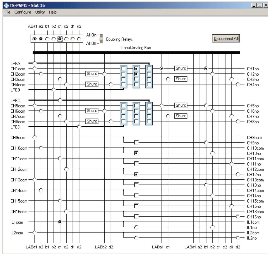
Figure 7-1 Softpanel R&S TS-PSM1 (example)
