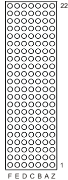
Figure 9-5 Connector X20 (mating side)
