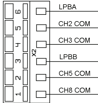
Figure 9-2 Terminal X2
