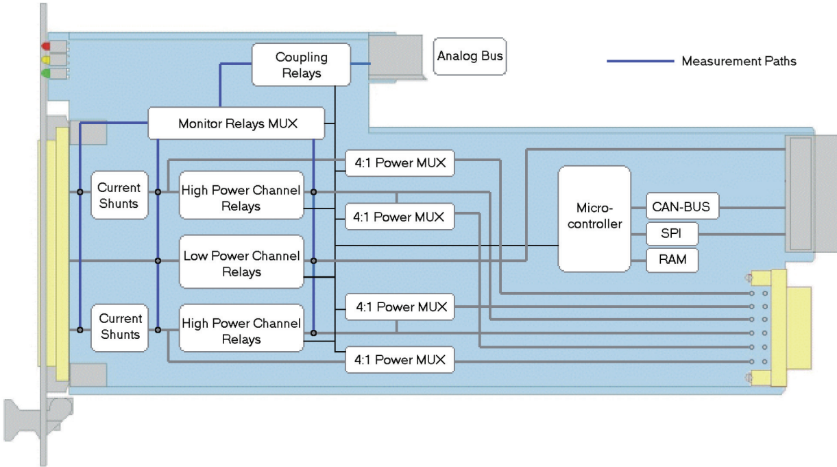
Figure 3-2 Functional Block Diagram R&S TS-PSM1
