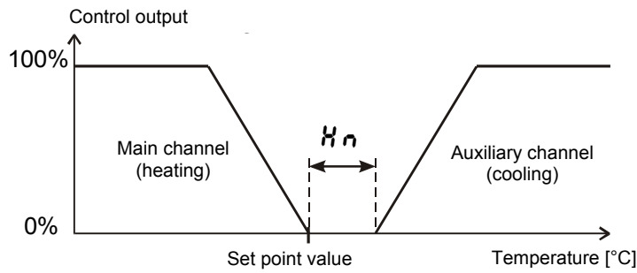
Fig.21. Control with two channels – heating-cooling type
