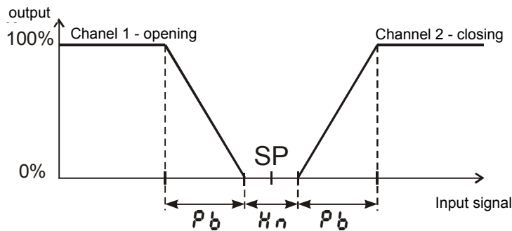
Fig. 18. three-stage step-by-step control
