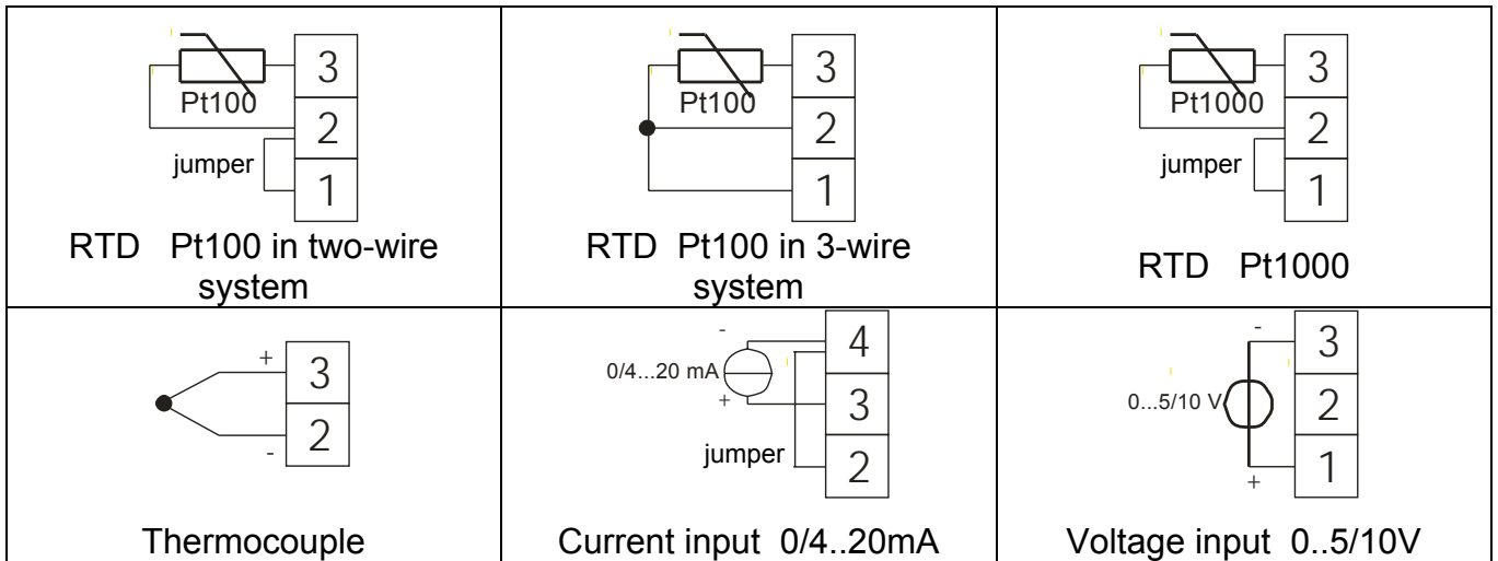
Fig. 5. Input signals
