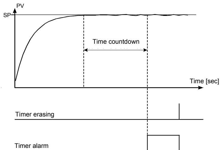
Fig.23. Principle of timer operation
