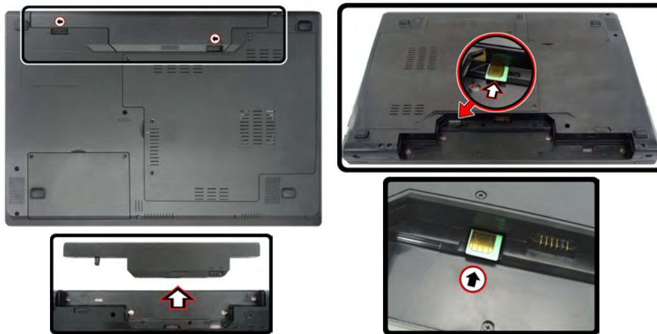
Figure 1 - 7 - Battery Removal & USIM Card Insertion
