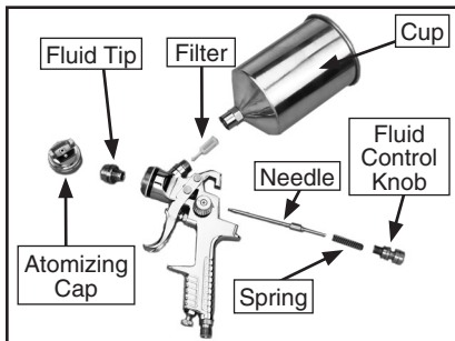
Figure 13. Disassembly for cleaning.
