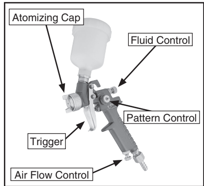
Figure 3. Controls.
