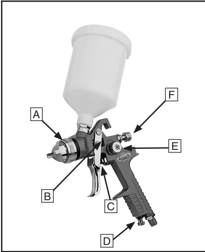
Figure 14. Lubrication points.
