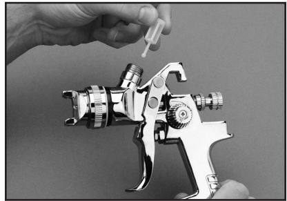
Figure 2. Installing filter.
