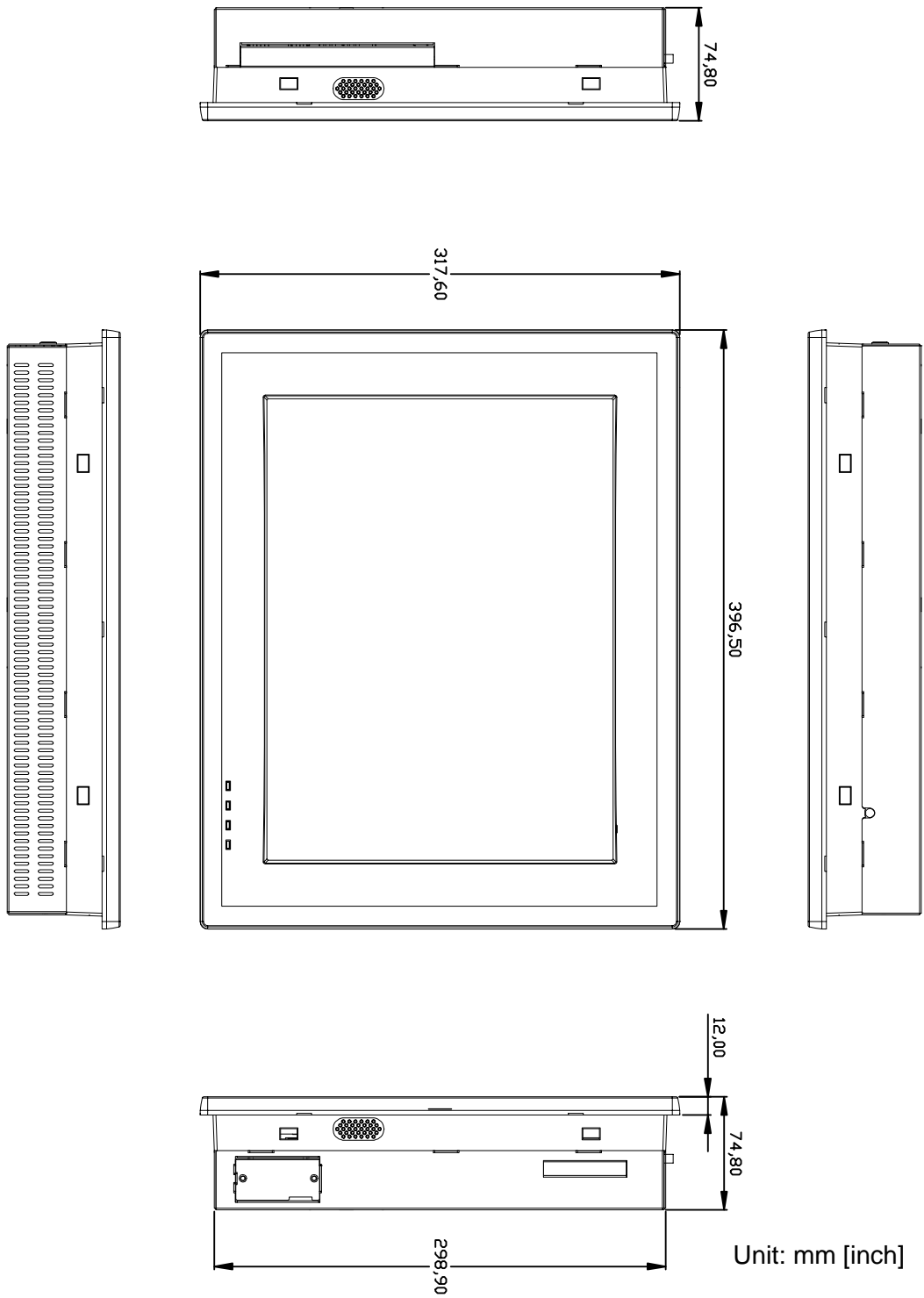
Figure 1.1 Dimensions of PPC-L157T
