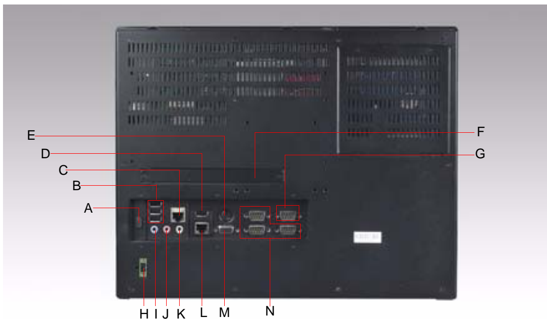
Figure 2.2 Rear view of Panel PC
