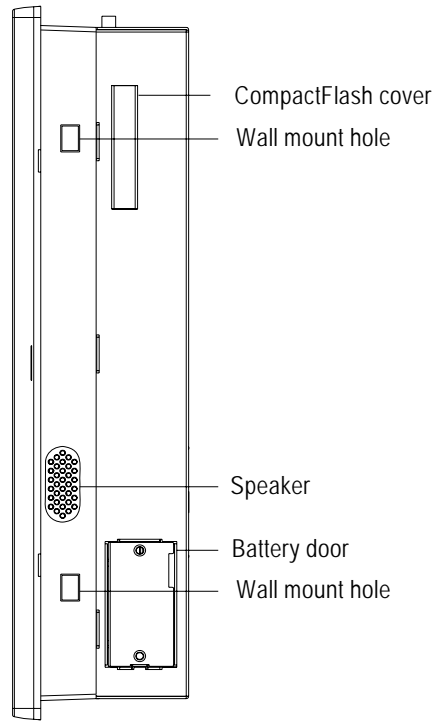
Figure 2.3 Side view of the panel PC
