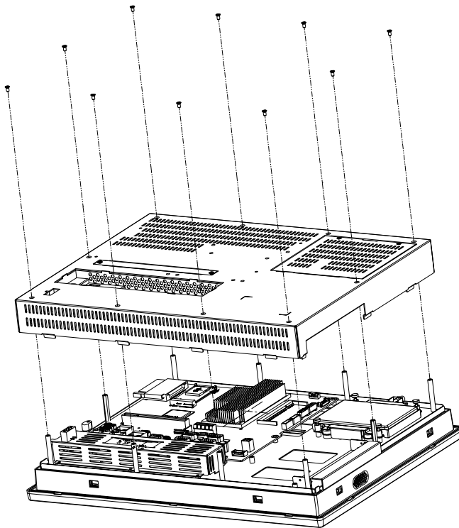
Figure 3.1 Installing primary 2.5" HDD
