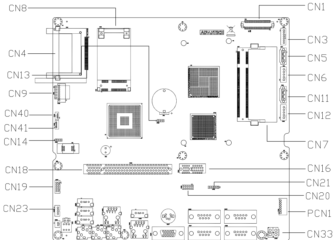
Figure 4.1 Jumpers and Connectors on the PPC-L157T motherboard
