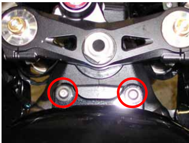
Figure 17 these screws have to be removed
