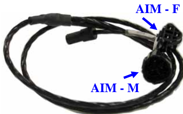
Figure 11: AIM TPS Cable
