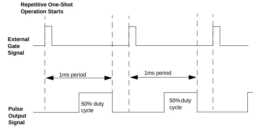
Figure 2-22 Example of repetitive one-shot mode using a 50% duty cycle
