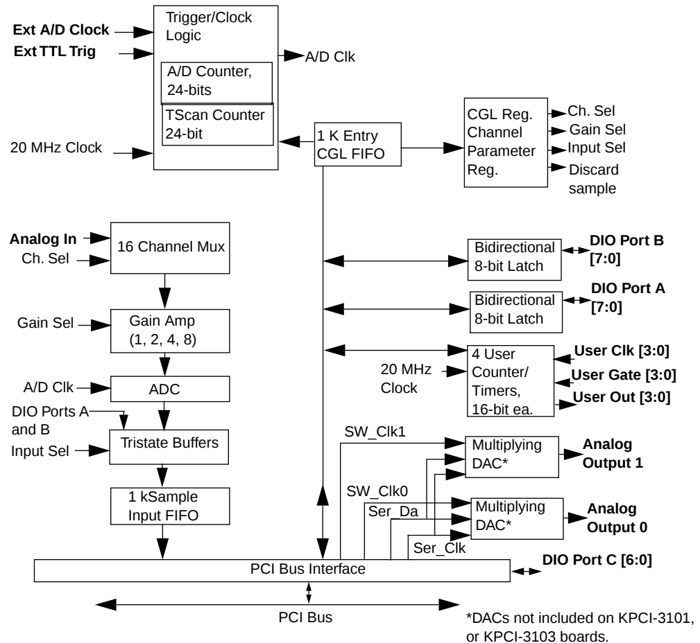
Block diagram of the KPCI-3101–4 series boards
