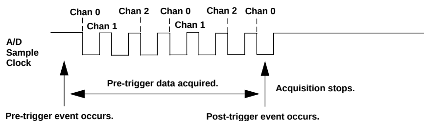
Figure 2-4 Continuous pre-trigger mode
