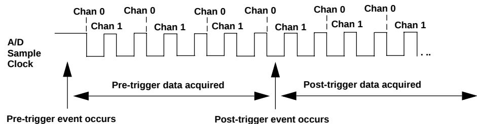
Figure 2-6 Continuous about-trigger mode
