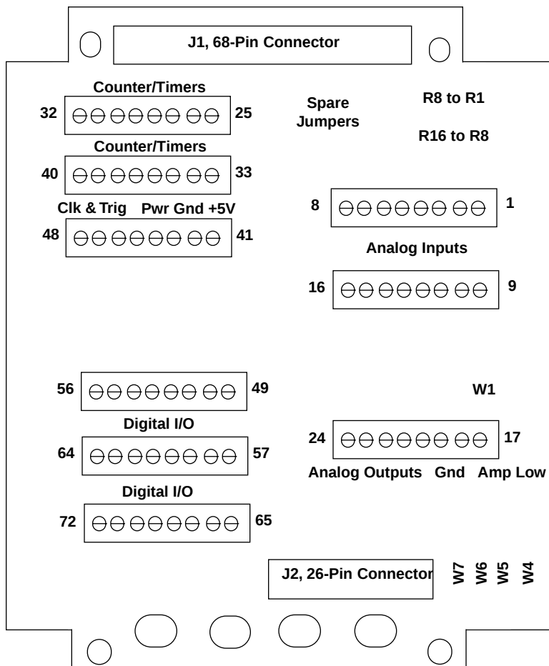
Layout of the STA-300 screw terminal panel
