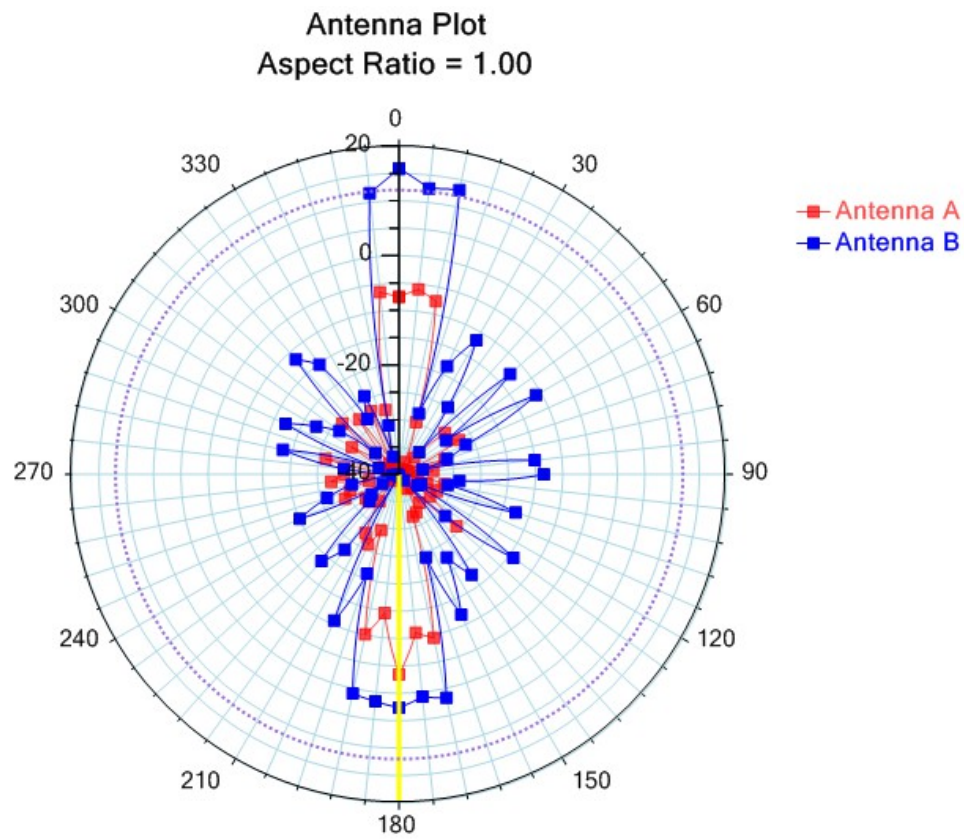
Antenna chart
