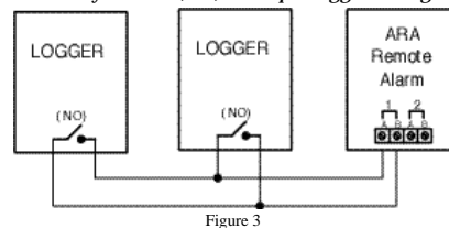
Normally Open (NO) multiple logger configuration
