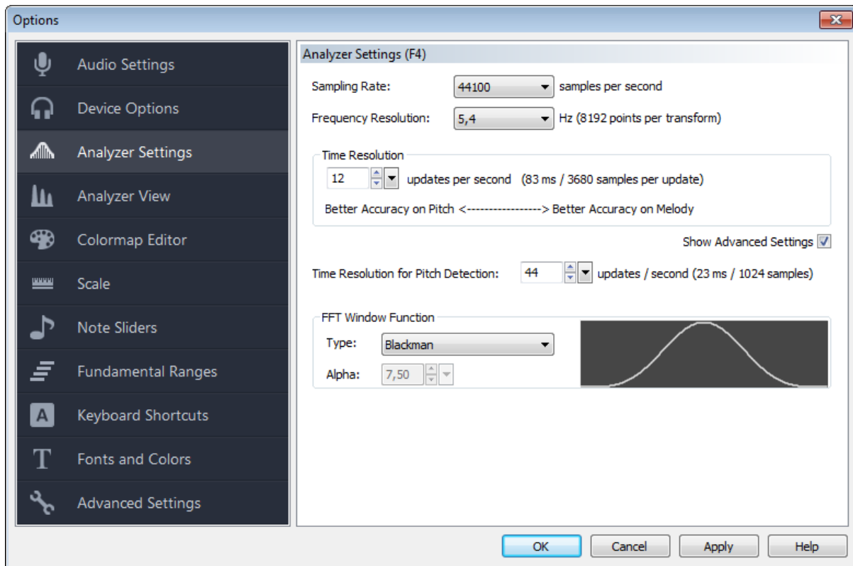
Figure 4.32. Analyzer Settings
