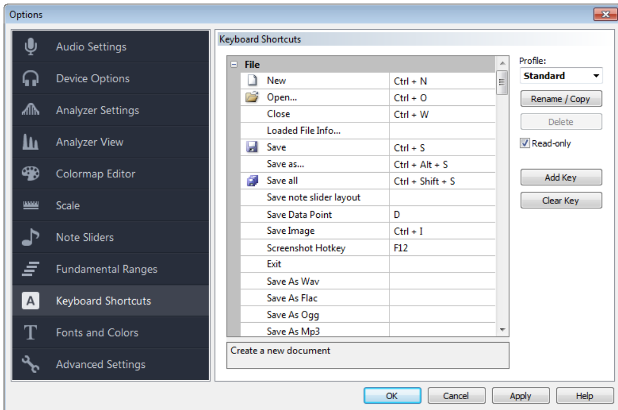
Figure 4.43. Keyboard shortcuts
