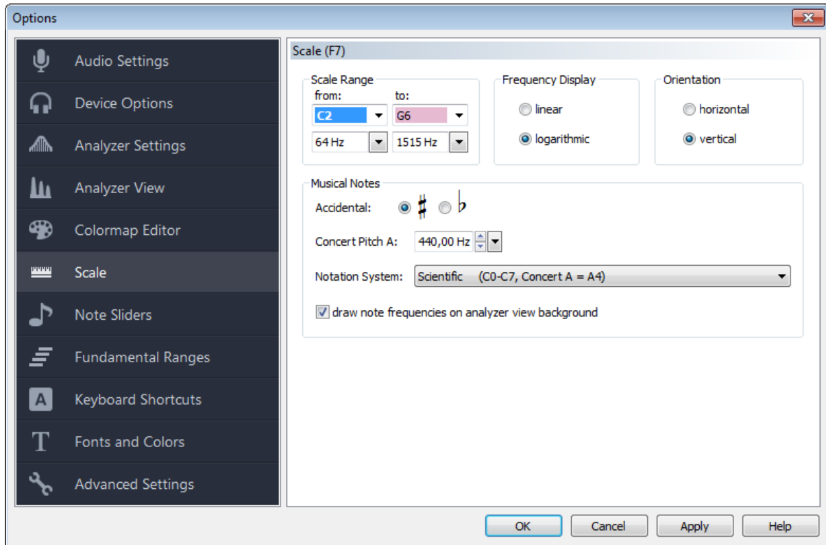
Figure 4.37. Scale Settings
