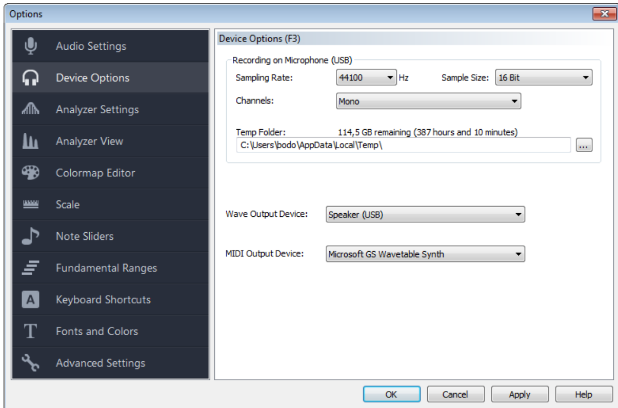
Figure 4.31. Device Options
