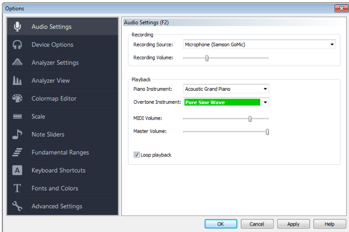
Figure 4.26. Audio Settings
