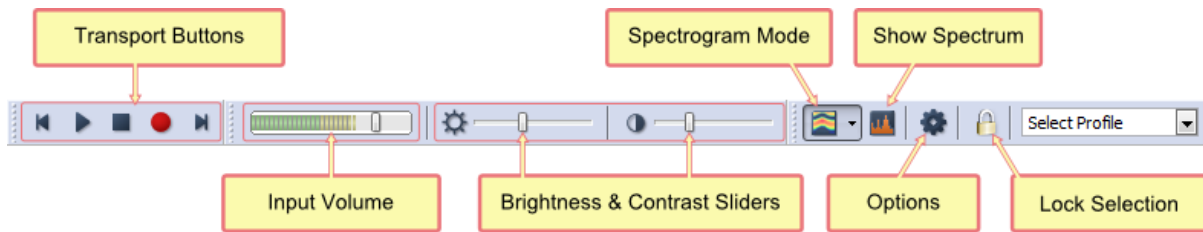
Figure 3.3. Toolbar buttons
