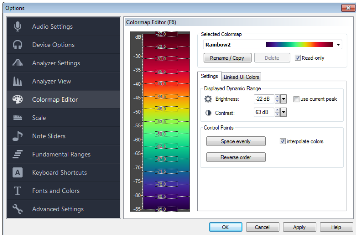
Figure 4.34. Colormap Editor
