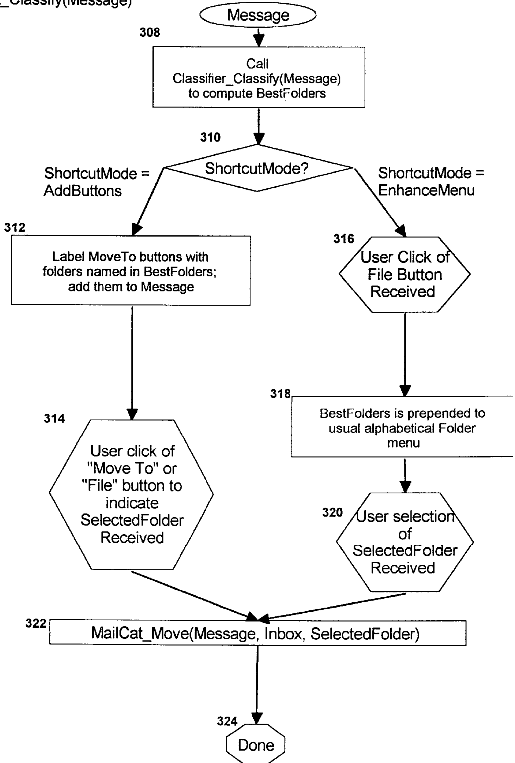
Figure 3 MailCat_Classify(Message)
