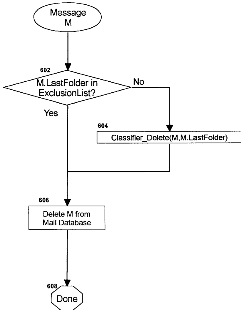
Figure 6 MailCat_Delete(Message)
