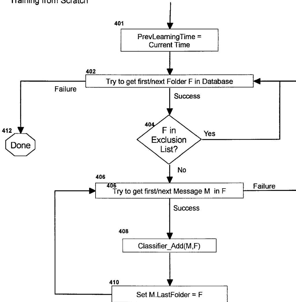
Figure 4 Training from Scratch
