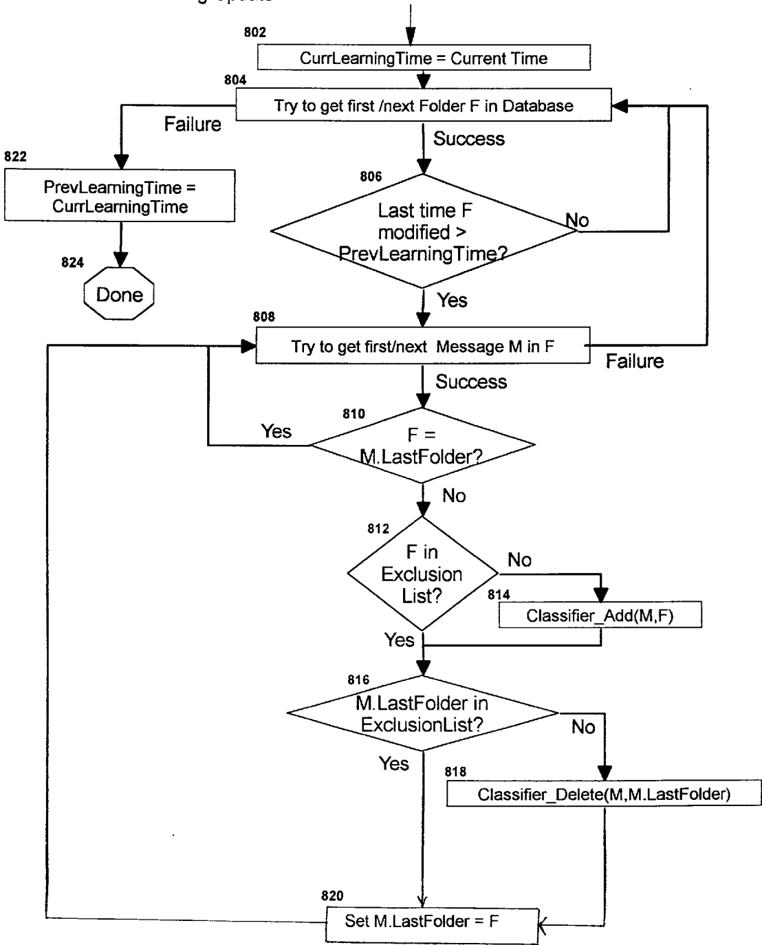
Figure 8 Incremental Learning Update
