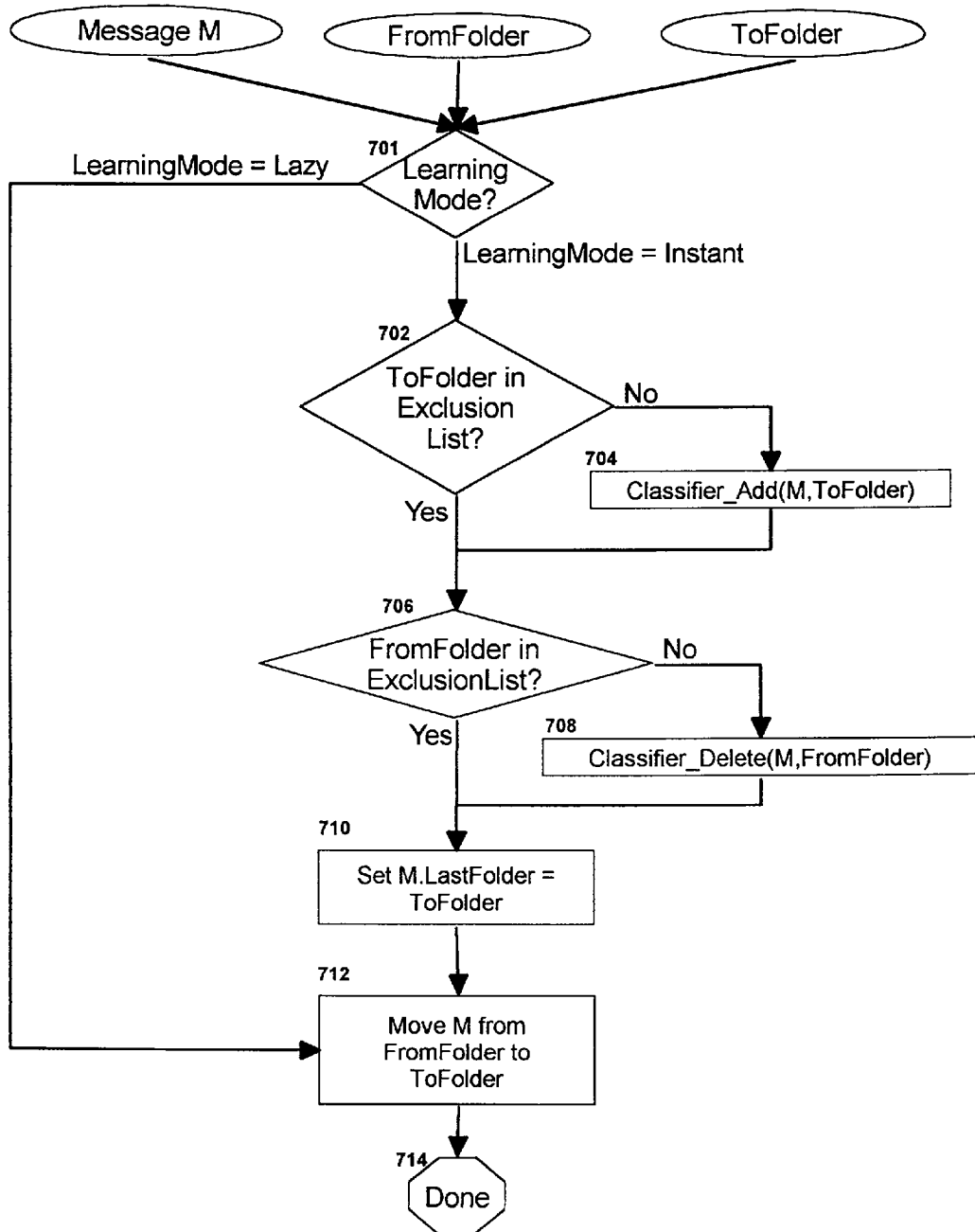
Figure 7 MailCat_Move(Message, FromFolder, ToFolder)
