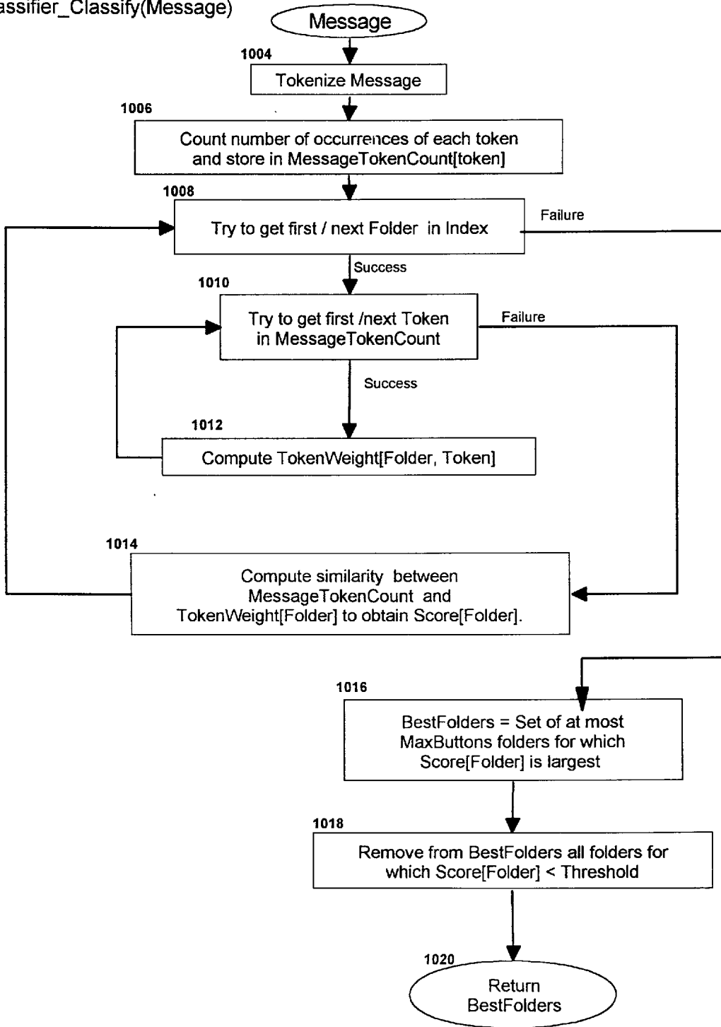
Figure 10 Classifier_Classify(Message)
