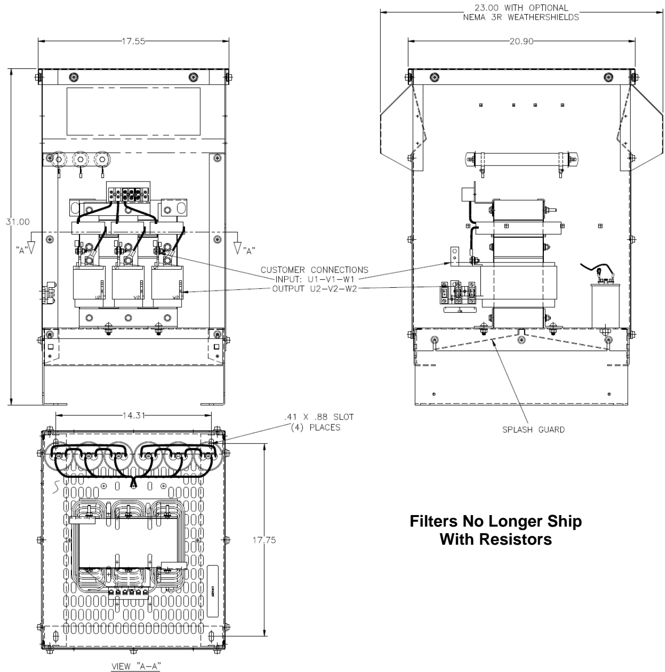
Figure 18 44-66 AMP
