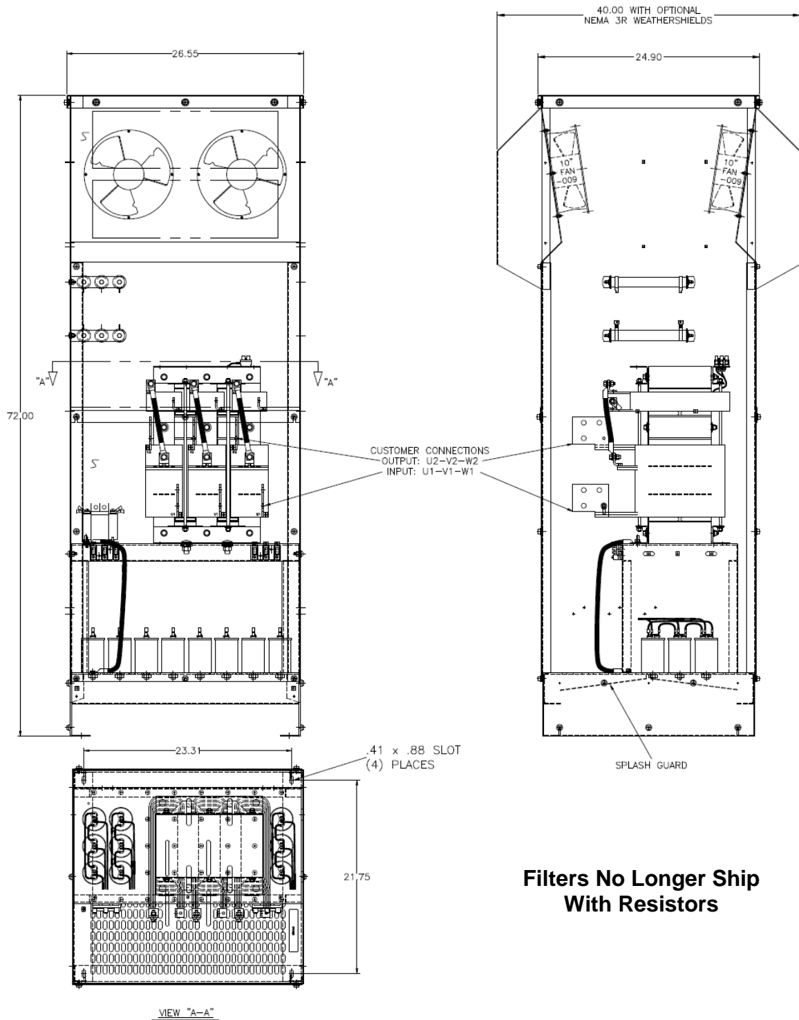
Figure 20 240-403 AMP
