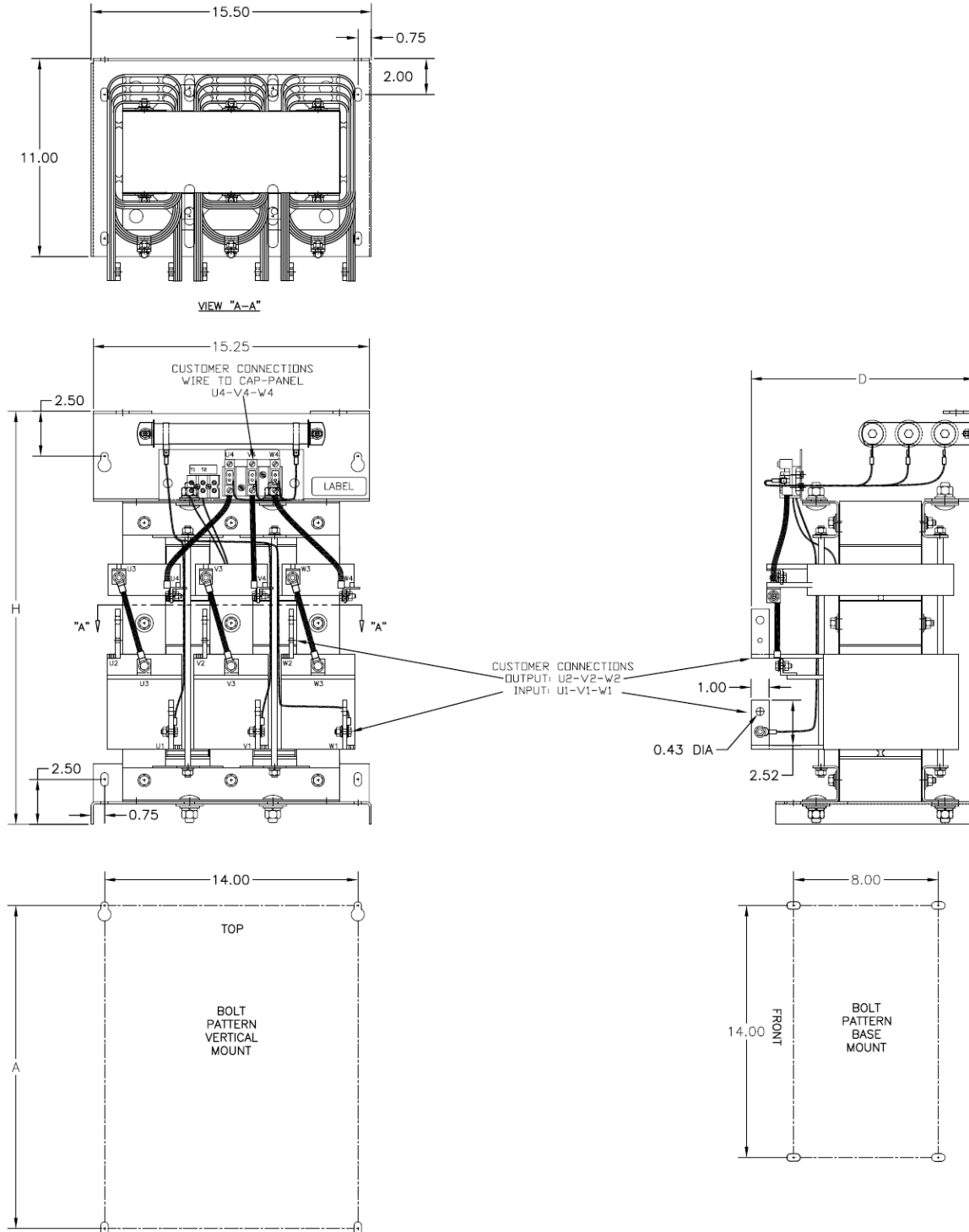
Figure 7 44 – 83 AMP
