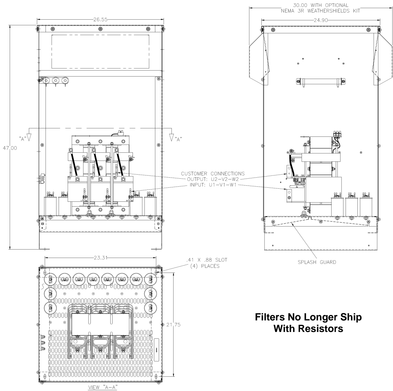
Figure 19 83-208 AMP
