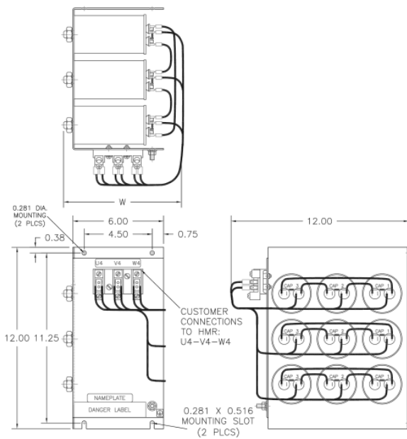
Figure 14 9 Caps
