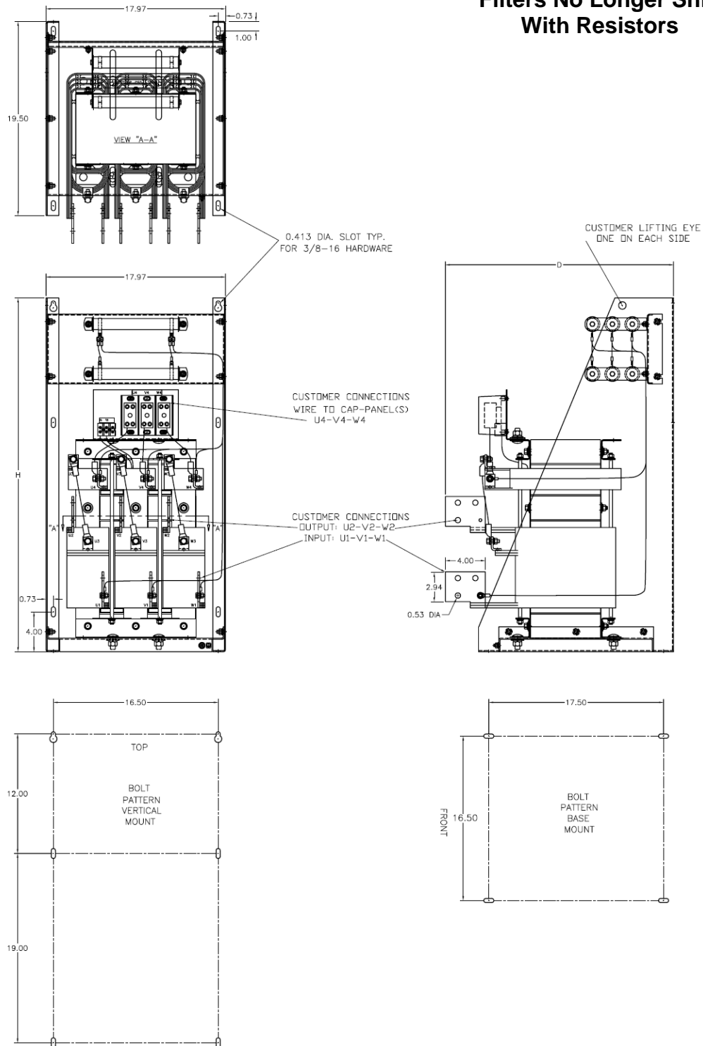
Figure 8 103 – 208 AMP
