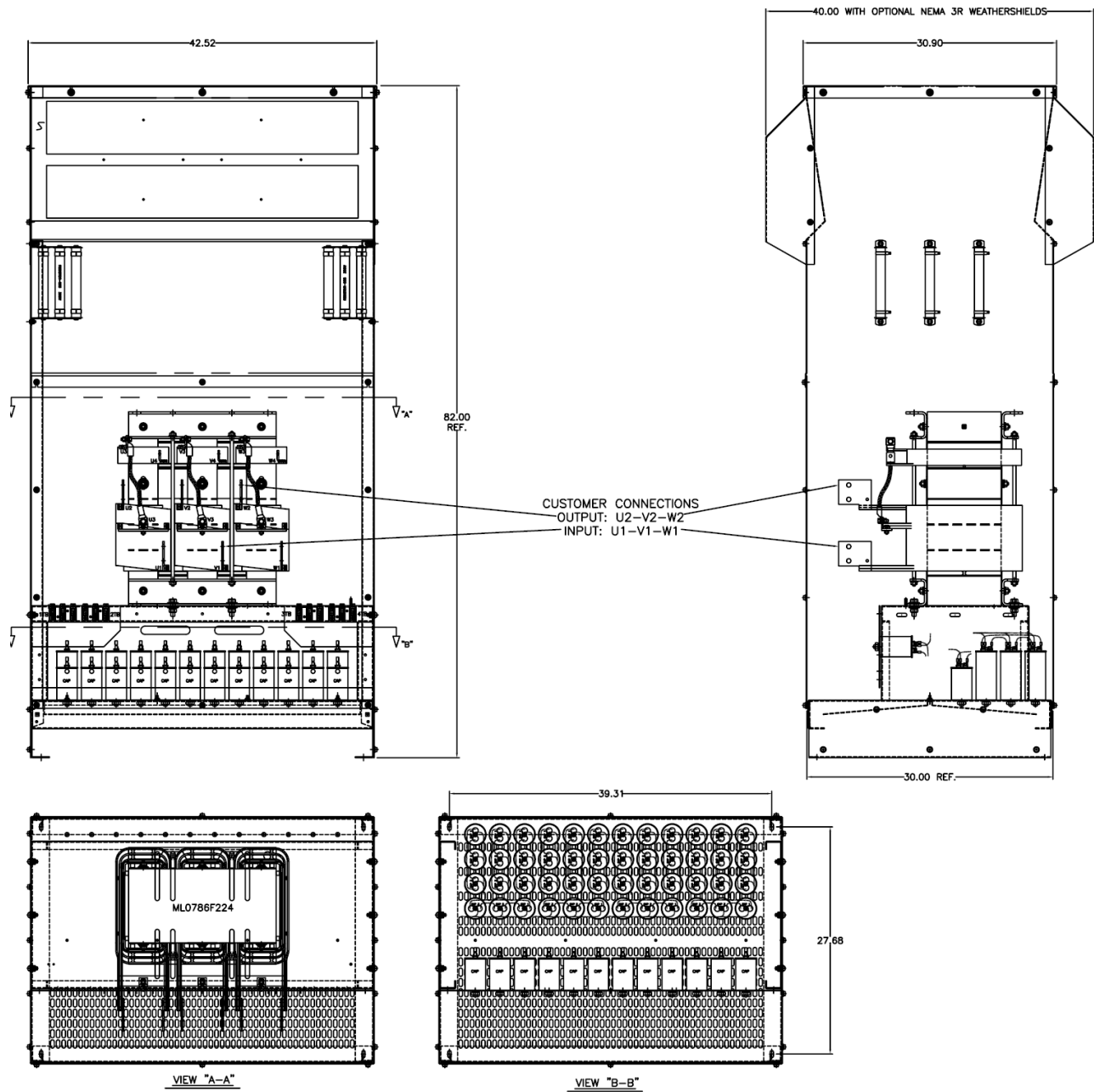
Figure 22 786 AMP
