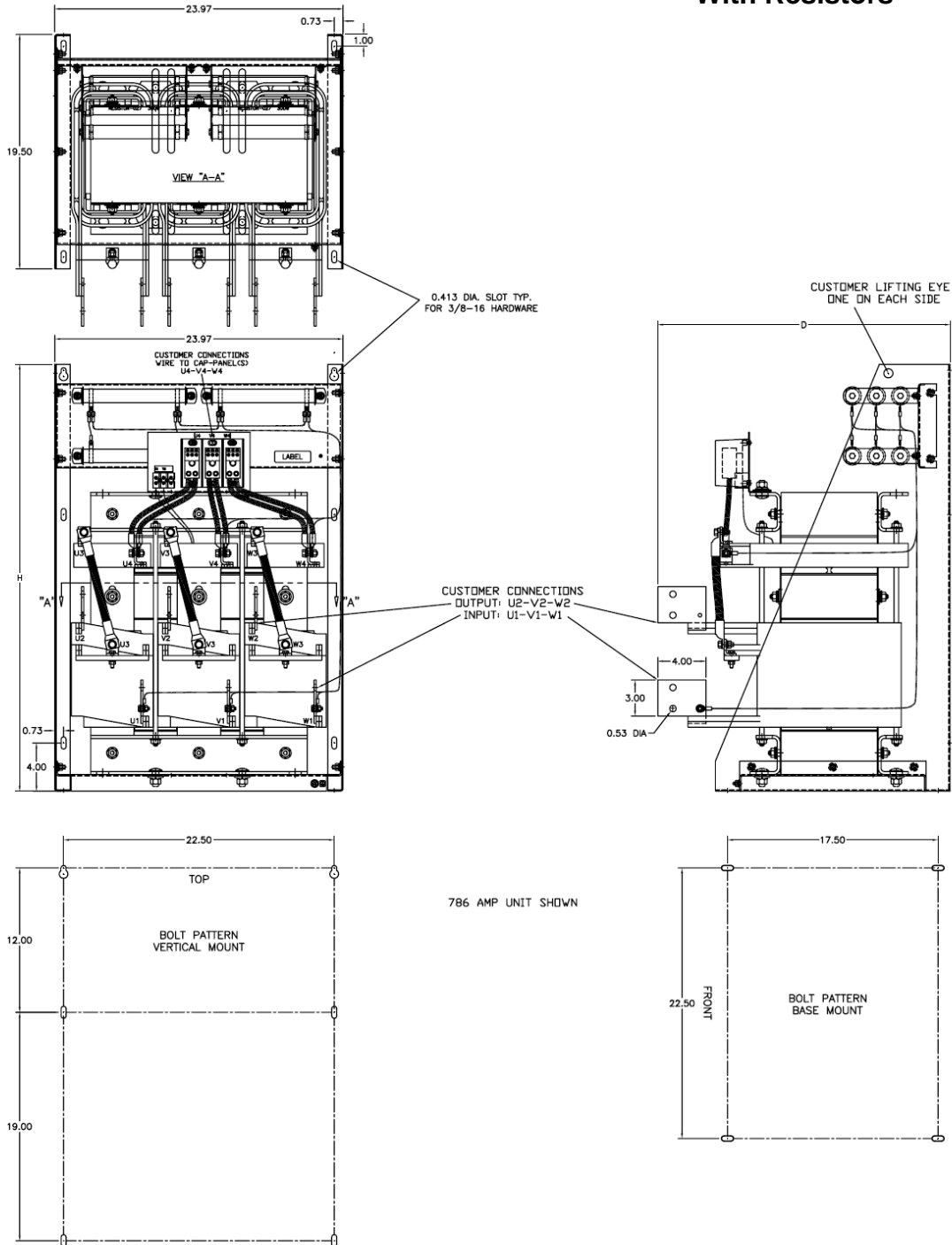
Figure 9 240 – 786 AMP
