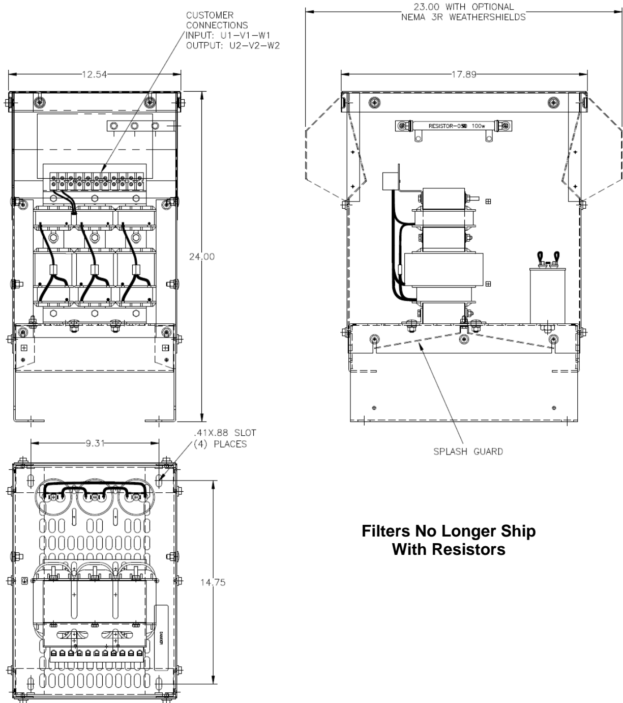
Figure 17 6 - 34 AMP
