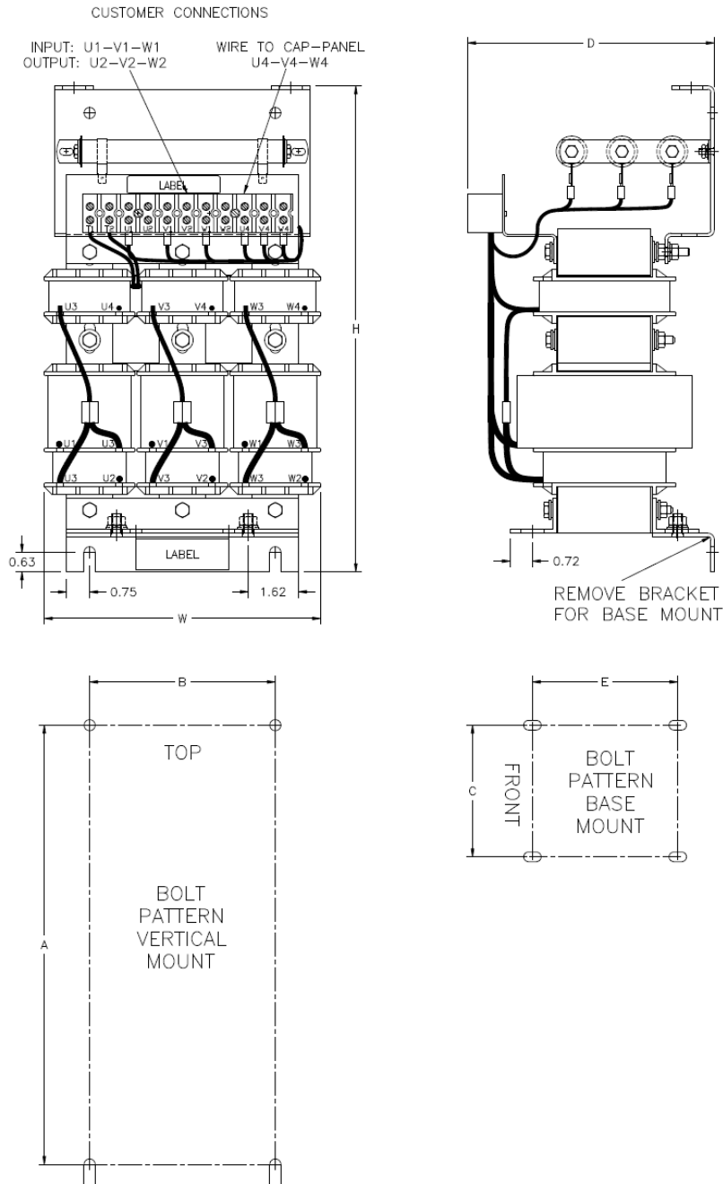
Figure 5 6 - 11 AMP
