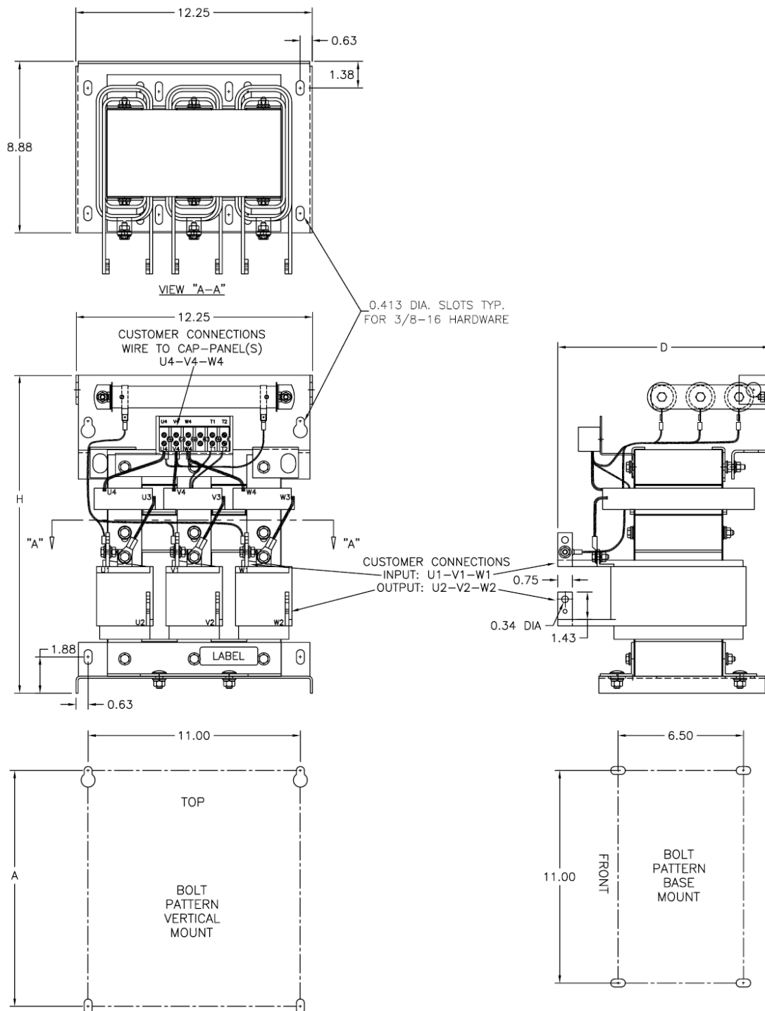
Figure 6 14 - 34 AMP
