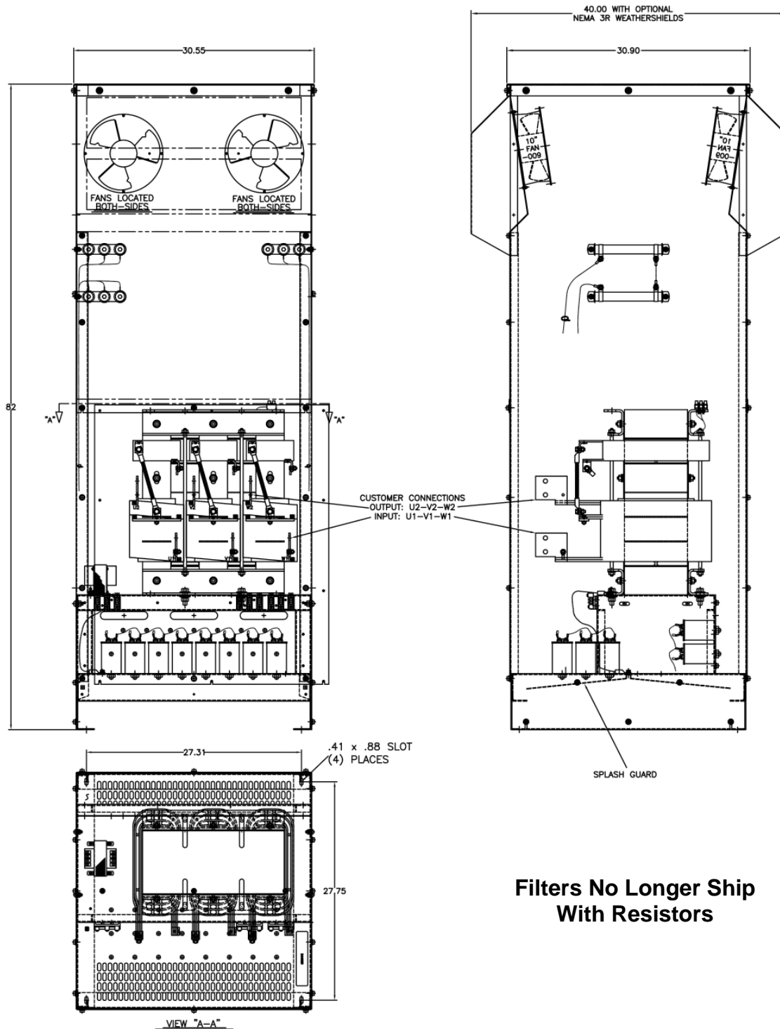
Figure 21 482-636 AMP
