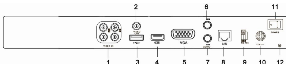
Figure 1.6 Rear Panel of DS-7204HVI/HFI/HWI-SH, DS-7204HVI-SV and DS-7204HWI-SV
