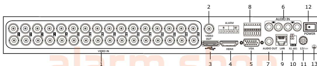
Figure 1.9 Rear Panel of DS-7232HVI-SH and DS-7232HWI-SH
