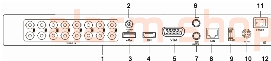
Figure 1.7 Rear Panel of DS-7216HVI-SH and DS-7216HVI-SV
