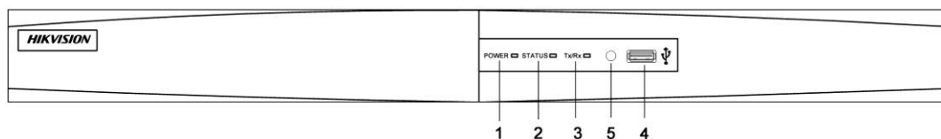
Figure 1.1 Front Panel of DS-7200-SH/SV
