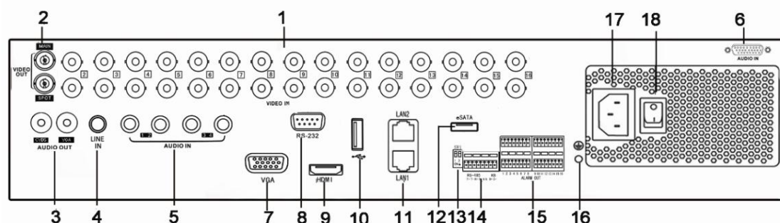
Figure 1.12 Rear Panel of DS-8132HCL-SH, DS-8132HFSI-SH and DS-8132HWSI-SH
