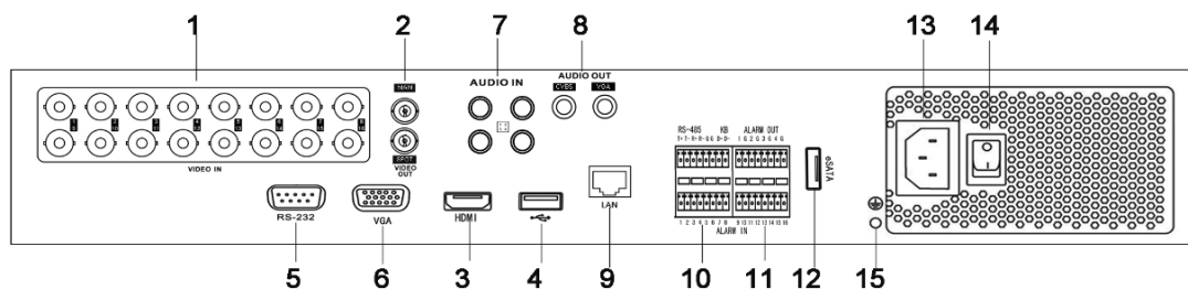
Figure 1.10 Rear Panel of DS-7316HFI-SH and DS-7316HWI-SH
