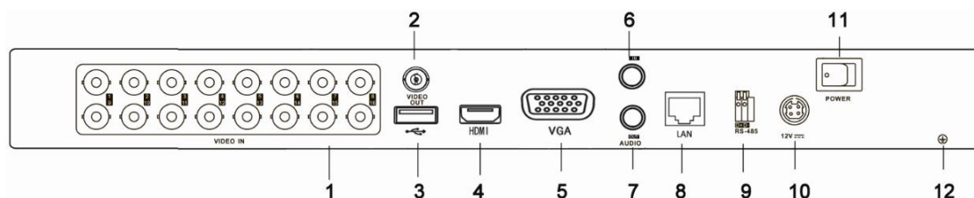
Figure 1.8 Rear Panel of DS-7216HFI-SH and DS-7216HWI-SH
