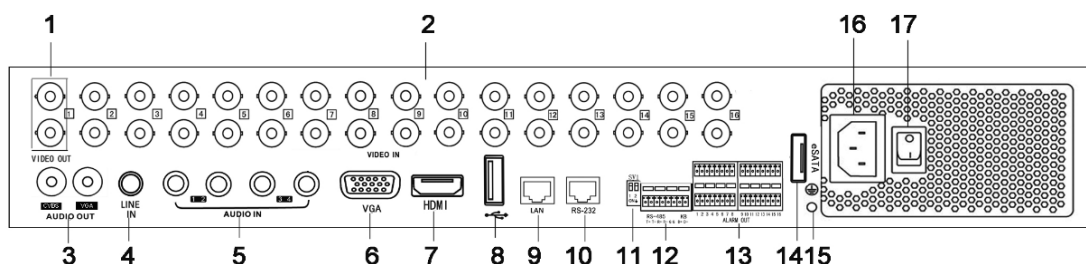
Figure 1.11 Rear Panel of DS-7332HFI-SH, DS-7332HWI-SH and DS-7332HI-SH
