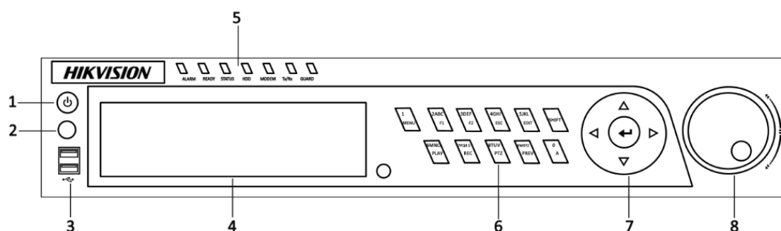
Figure 1.2 Front Panel of DS-7300-SH
