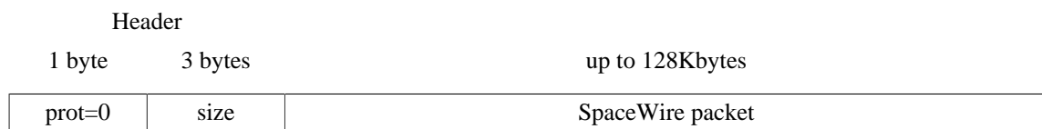
Figure 3.2. Transmit data format
