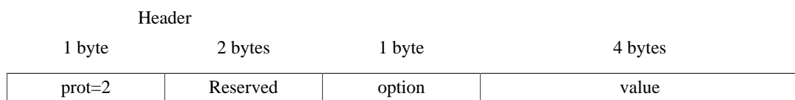
Figure 3.7. Status protocol format
