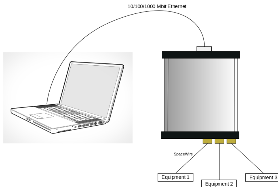
Figure 1.1. GRESB system diagram
