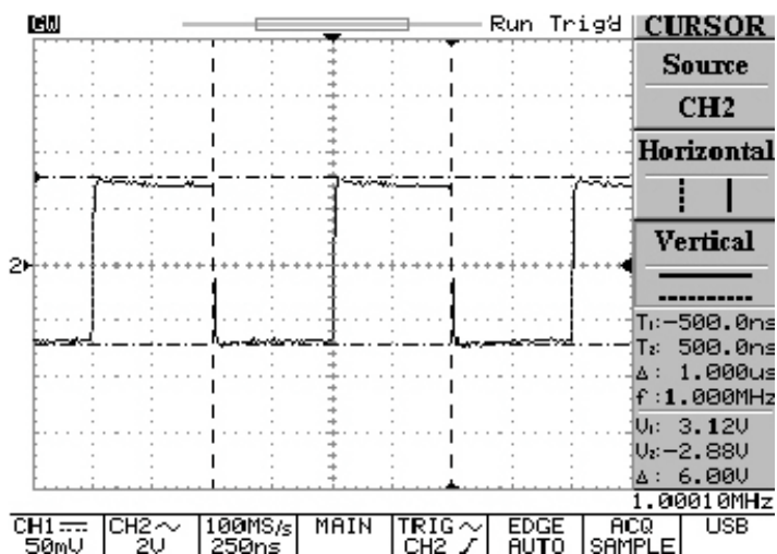
Figure 5-29: Adjusting the horizontal and vertical position for channel two inputs
