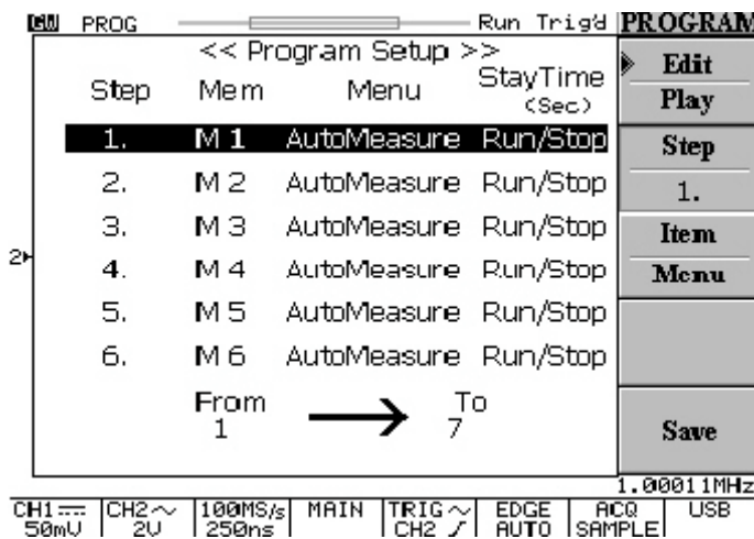
Figure 5-31: Enter to program mode
