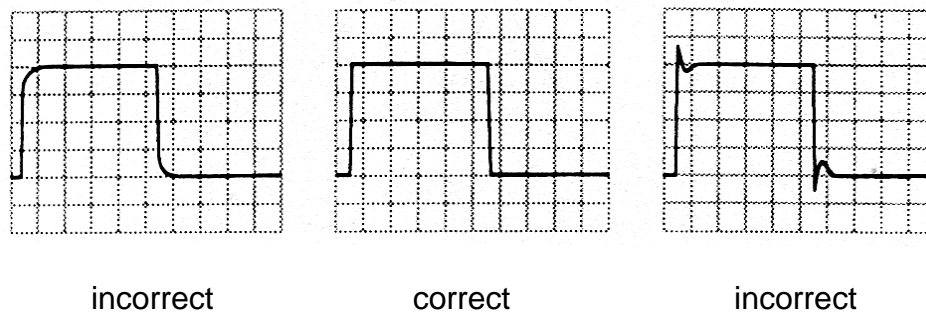
Figure 3-2: Probe compensations
