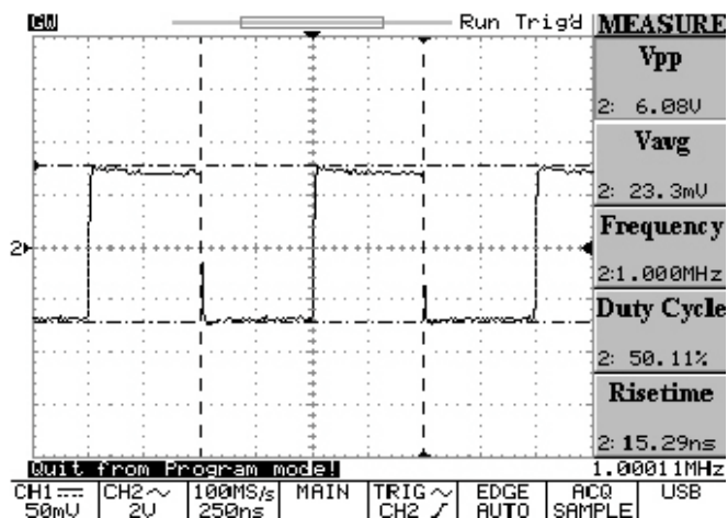
Figure 5-38: Quit the program mode by pressing AUTO TEST/STOP button
