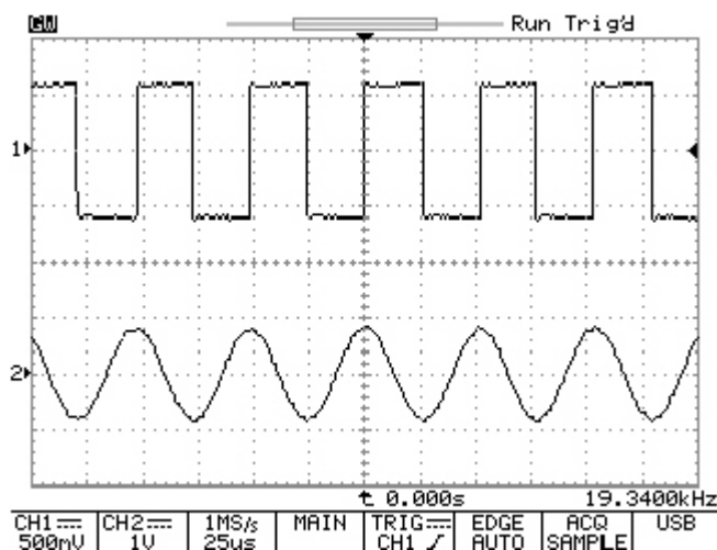
Figure 5-43: A large twelve division waveform display without side menu.
