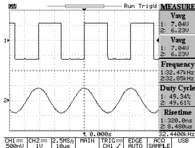
Figure 5-40: 10 measurements are displayed in the same time
