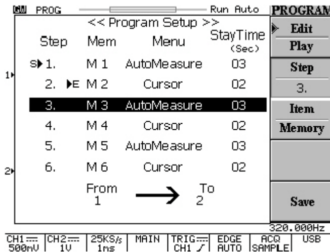
Figure 5-25: Press PROGRAM pushbutton and enter to “Program” mode
