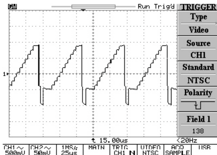
Figure 5-15: Vide trigger mode
