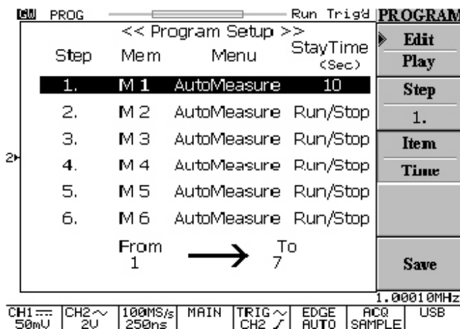
Figure 5-32: Editing the program condition of step one
