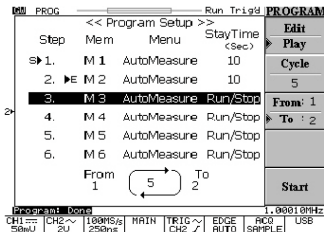
Figure 5-37: the Entire program running is finished
