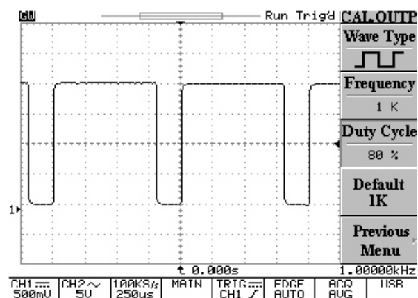
Figure 5-24: The menu for adjustable probe compensation signal
