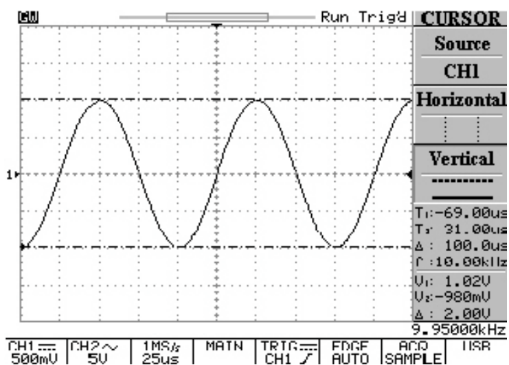
Figure 5-27: Adjusting the vertical position for channel one input of example
