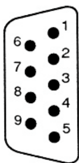
Figure 7-1: Pin assignment for the oscilloscope's RS232 connector
