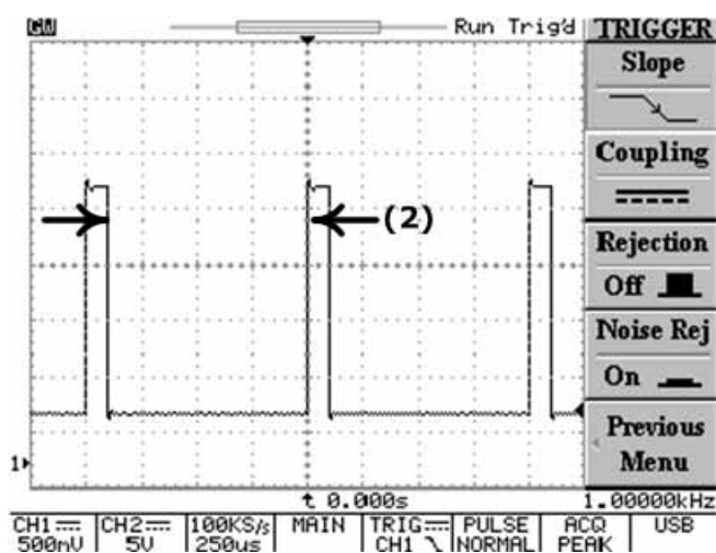
Figure 5-17: Pulse width trigger with negative polarity selected
