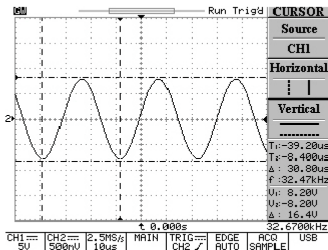
Figure 5-39: Vertical and horizontal cursors measurements
