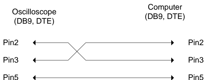
Figure 7-2: DB9 to DB9 wiring
