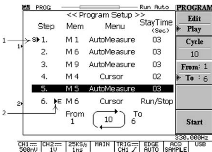
Figure 5-26: Programming for play function of “Program” mode
