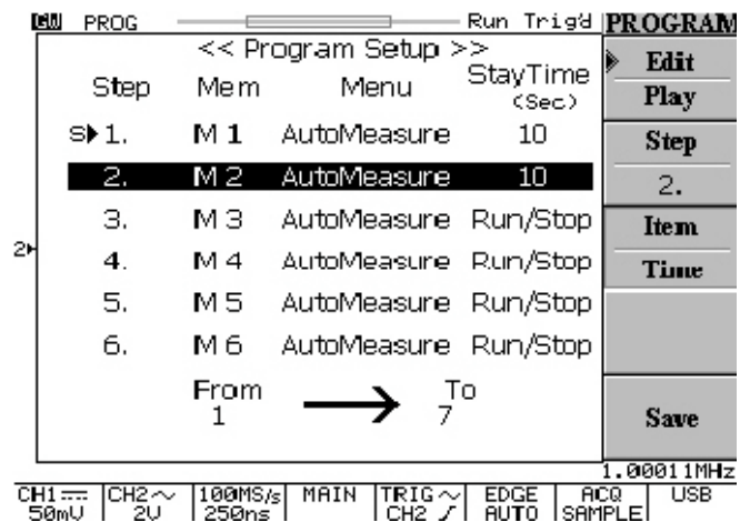
Figure 5-33: Editing the program condition of step two
