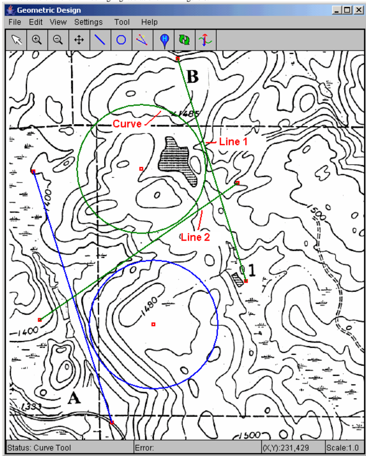
Figure 6 Select horizontal alignment elements
