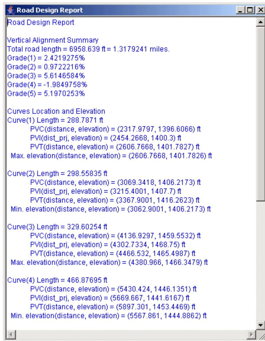
Figure 13 Report of roadway geometry design
