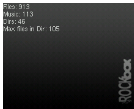
Figure 12.54.: The stats-plugin
