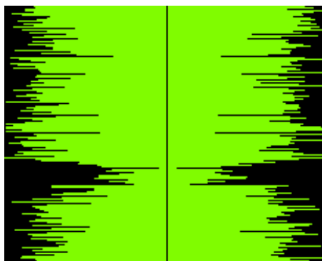
Figure 12.37.: Oscilloscope
