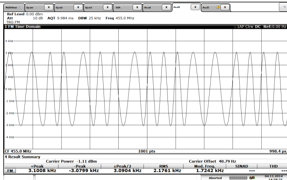
Figure 109 Tx Modulation V.23, 1200bps, I/Q Modulation
