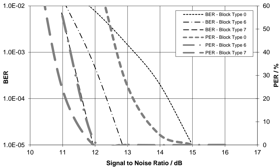
Figure 98 Comparison of BER and PER for 16-QAM Modulation
