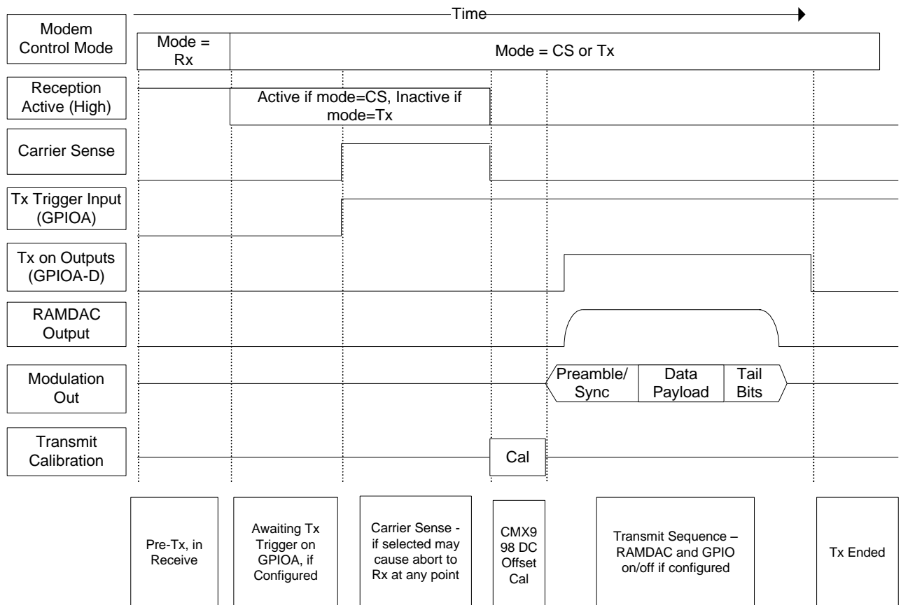
Figure 20 Transmit Sequence
