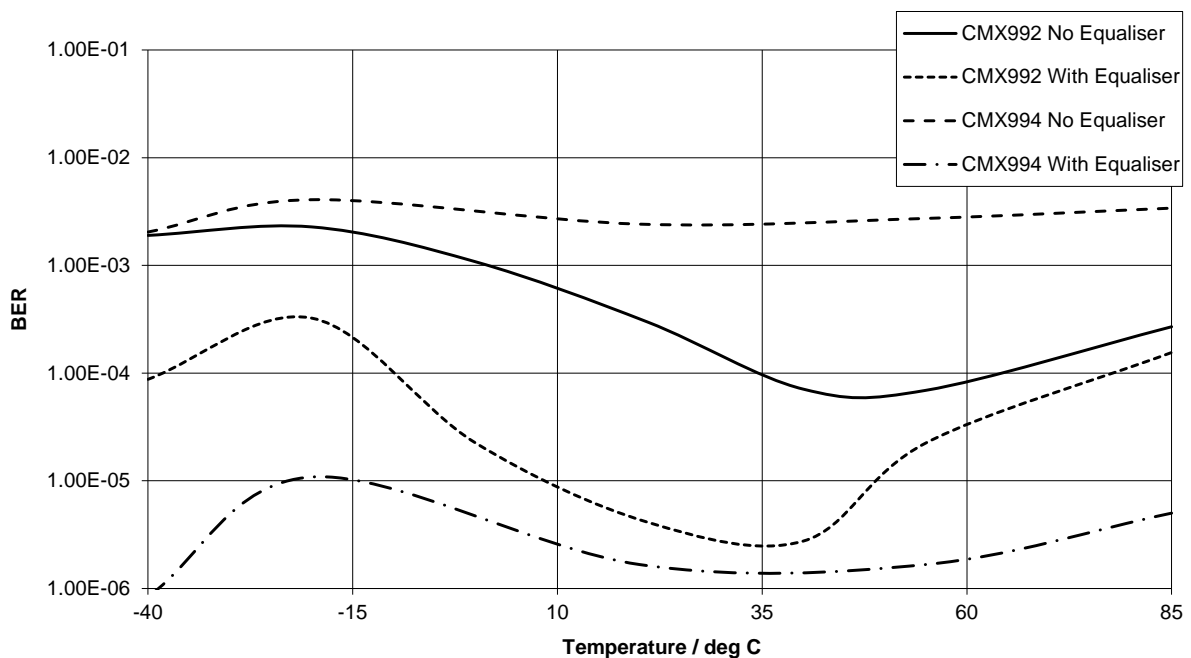
Figure 105 Performance of 16-QAM Equalised Signals with Temperature Variation and Constant Signal-to-Noise Ratio
