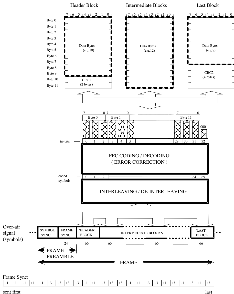
Figure 58 Native Formatted Data Over Air Signal Format
