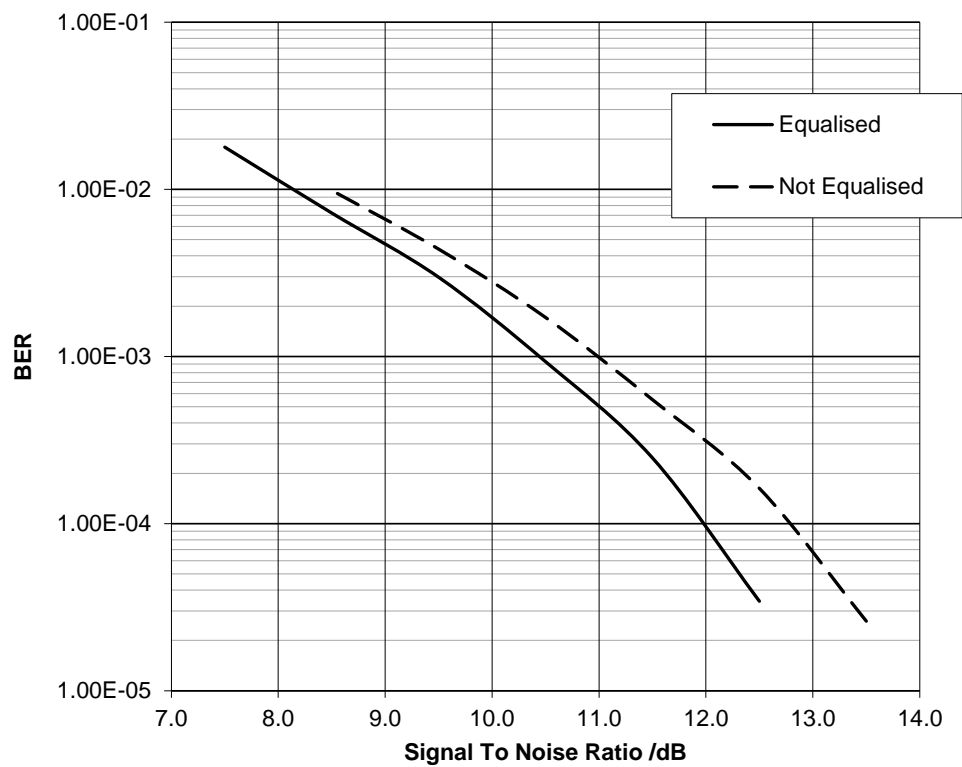
Figure 100 4-QAM Signal-to-Noise Performance, Equalised and Non-Equalised
