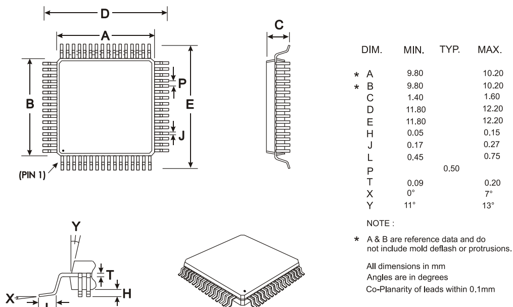
Figure 113 Mechanical Outline of 64-pin LQFP (L9)
