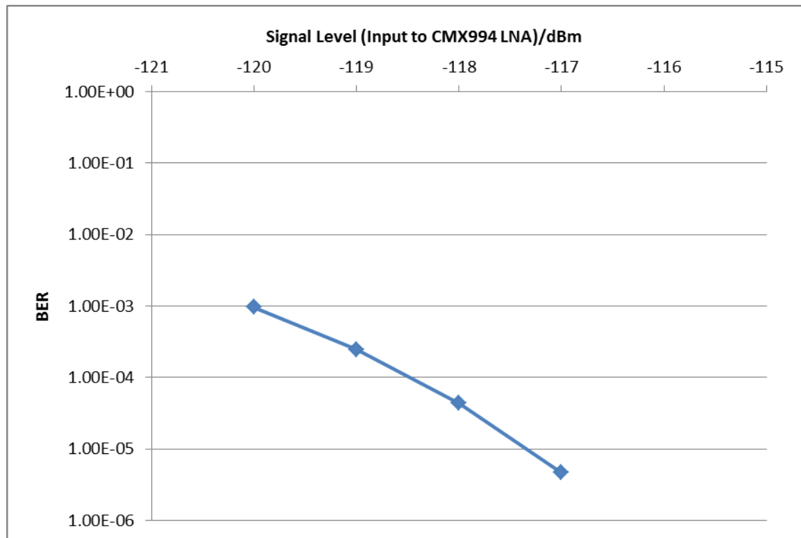
Figure 110 Signal Level vs BER
