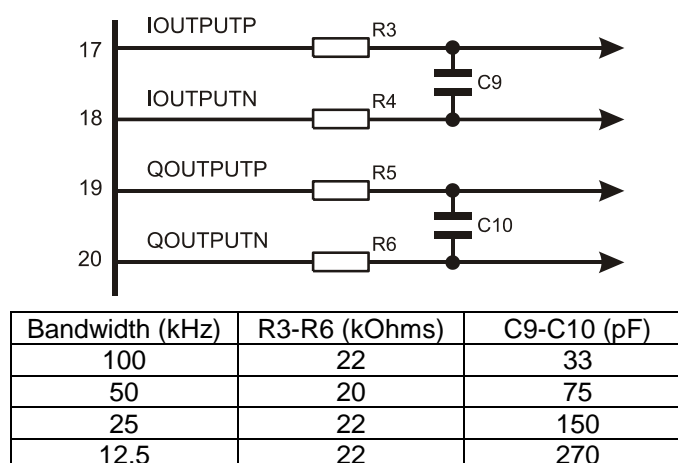
Figure 10 Recommended External Components – I/Q Output Reconstruction Filter
