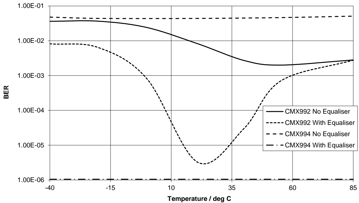
Figure 104 Performance of 64-QAM Equalised Signals with Temperature Variation
