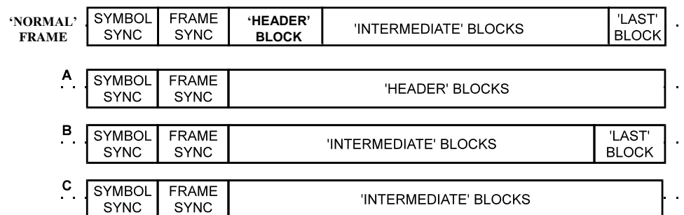
Figure 84 Suggested Frame Structures
