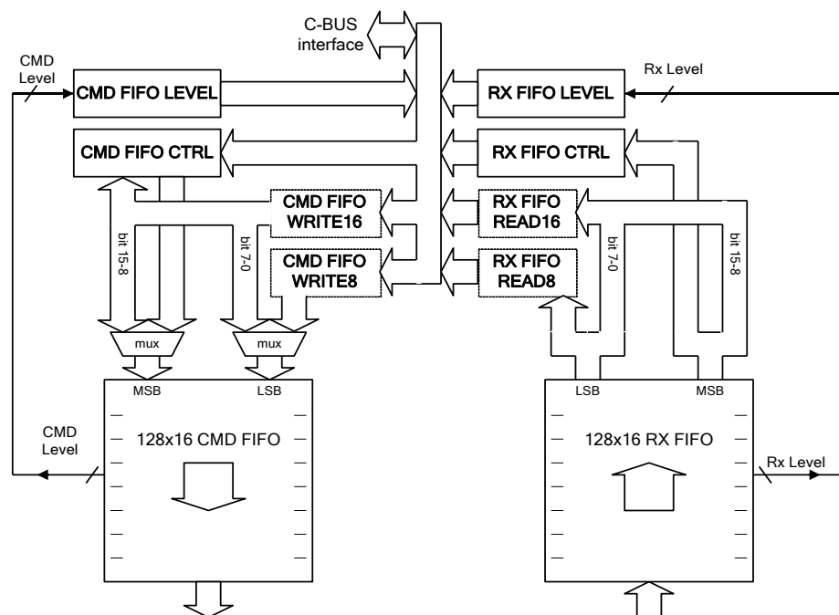
Figure 38 Command and Rx Data FIFOs
