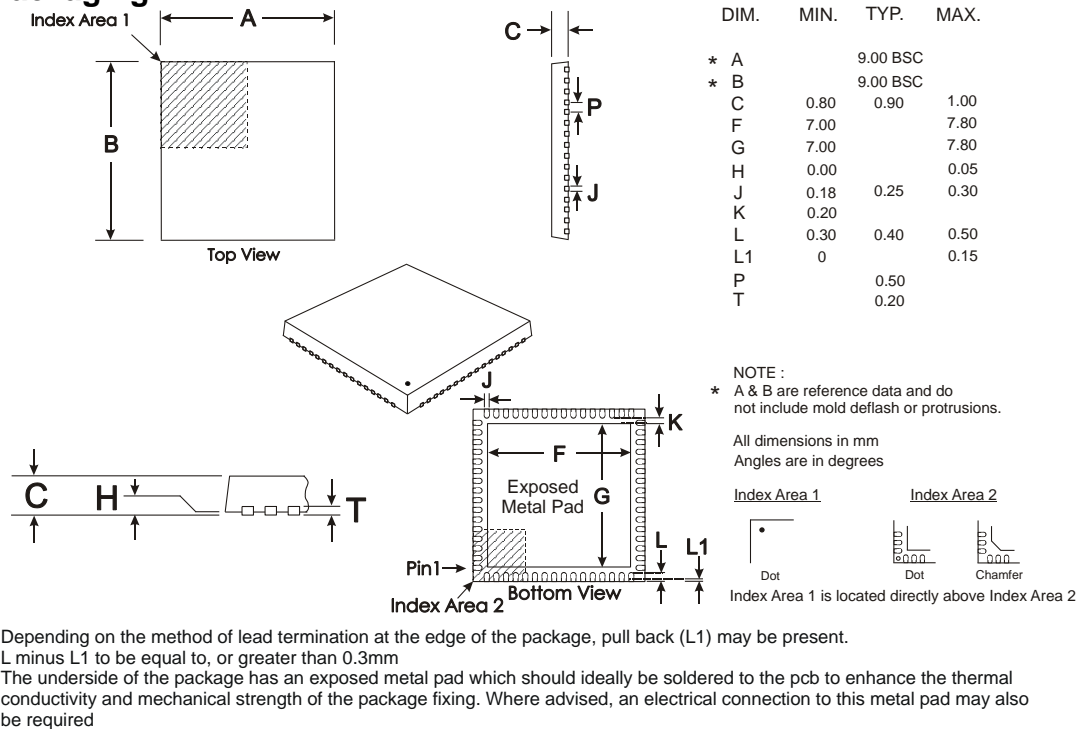
Figure 112 Mechanical Outline of 64-pin VQFN (Q1)
