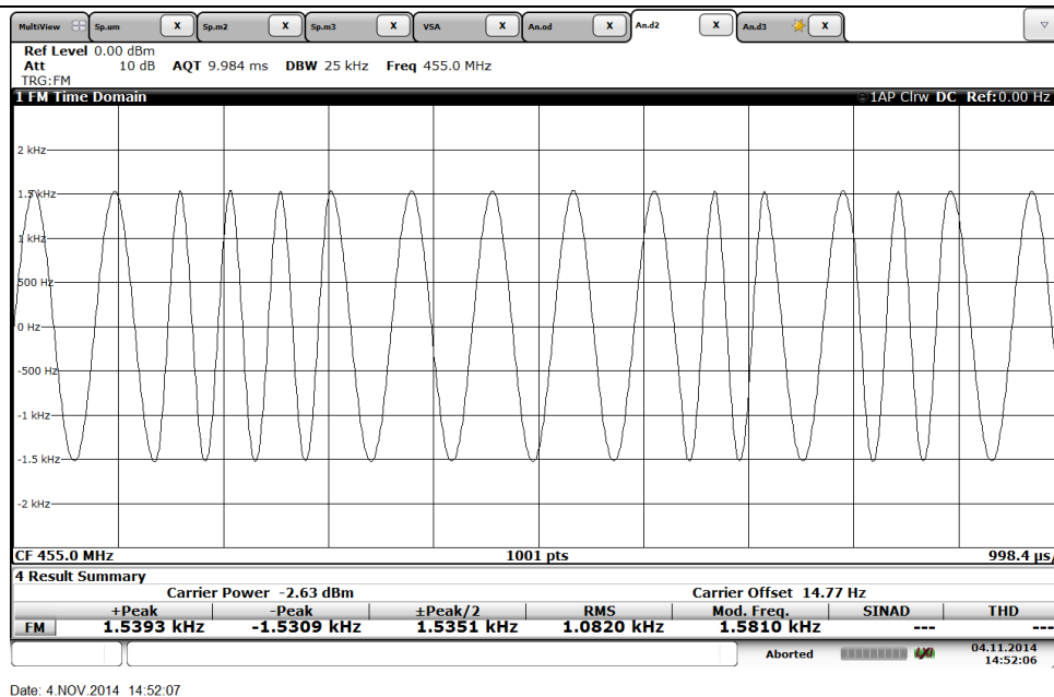
Figure 108 Tx Modulation V.23, 1200bps, I/Q Modulation
