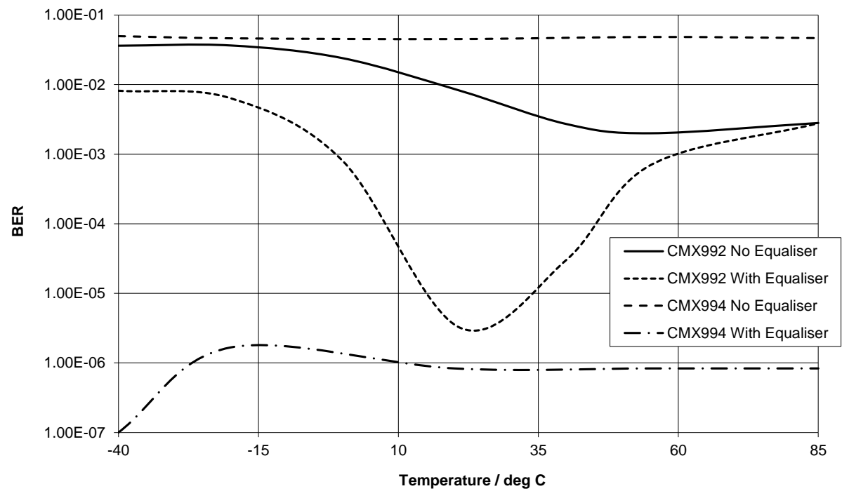
Figure 106 Performance of 64-QAM Equalised Signals with Temperature Variation and Constant Signal-to-Noise Ratio
