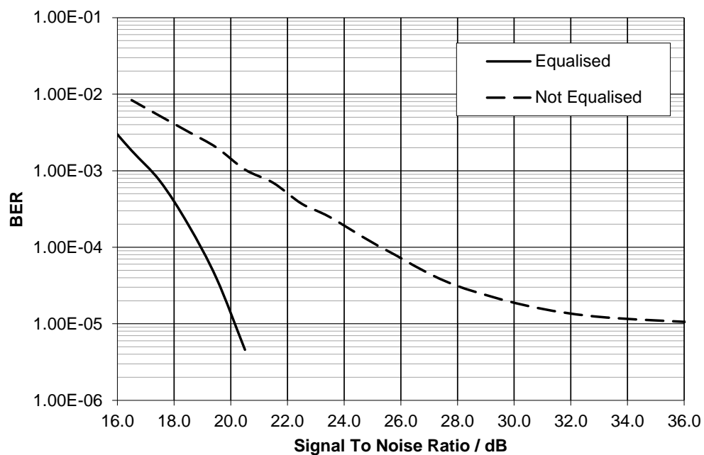
Figure 101 16-QAM Signal-to-Noise Performance, Equalised and Non-Equalised
