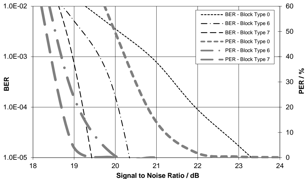
Figure 99 Comparison of BER and PER for 64-QAM Modulation
