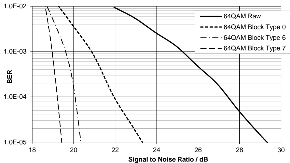
Figure 96 64-QAM Performance with Different Coding Schemes
