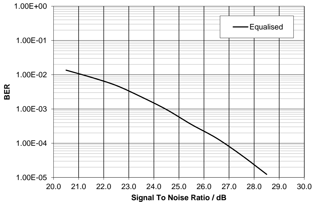
Figure 102 64-QAM Signal-to-Noise Performance, Equalised
