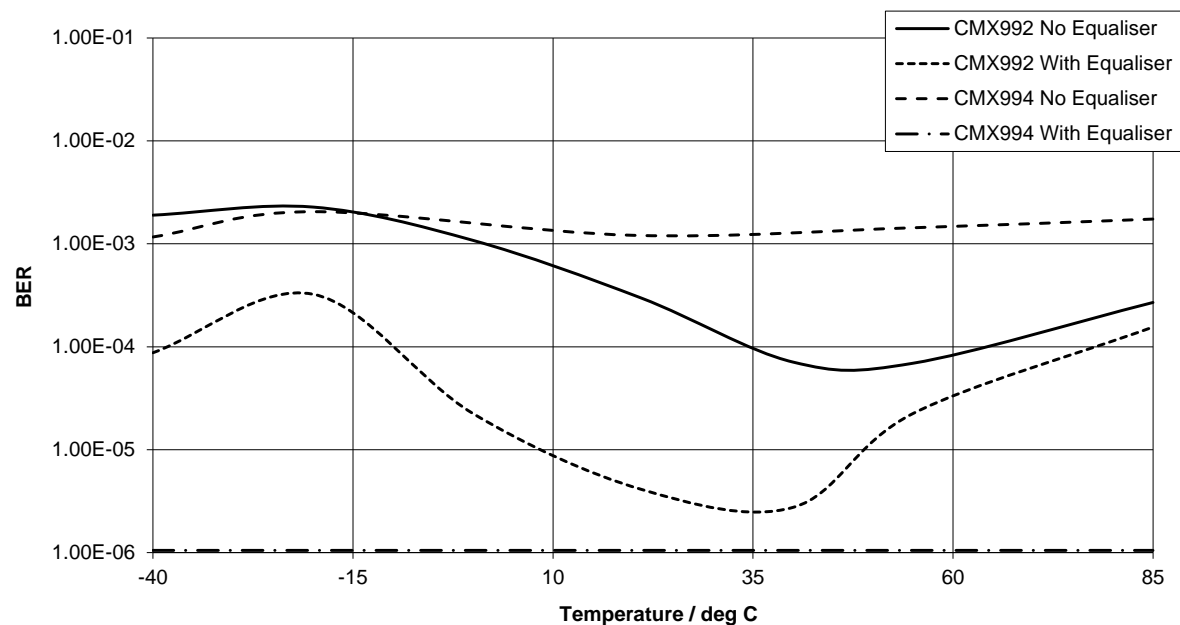
Figure 103 Performance of 16-QAM Equalised Signals with Temperature Variation
