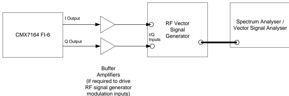
Figure 107 Tx Spectrum and Modulation Measurement Configuration for I/Q Operation
