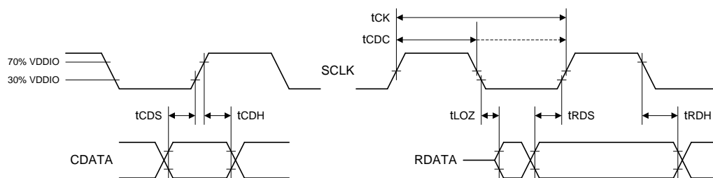
Figure 111 C-BUS Timing
