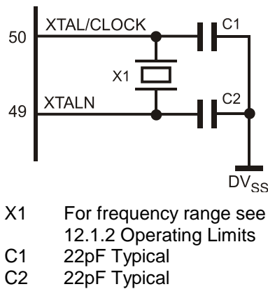
Figure 8 Recommended External Components – Xtal Interface
