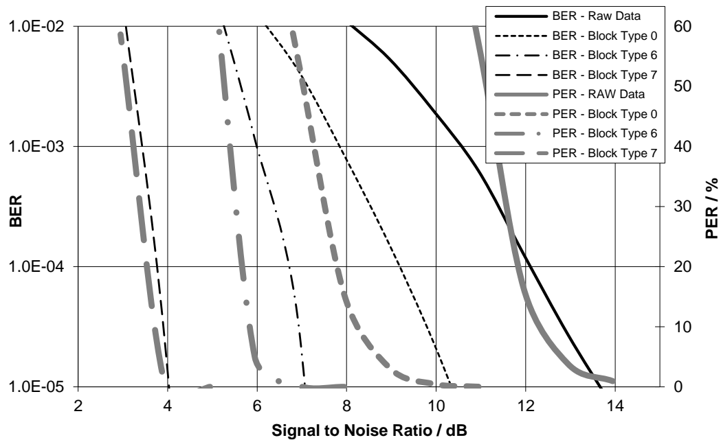
Figure 97 Comparison of BER and PER for 4-QAM Modulation
