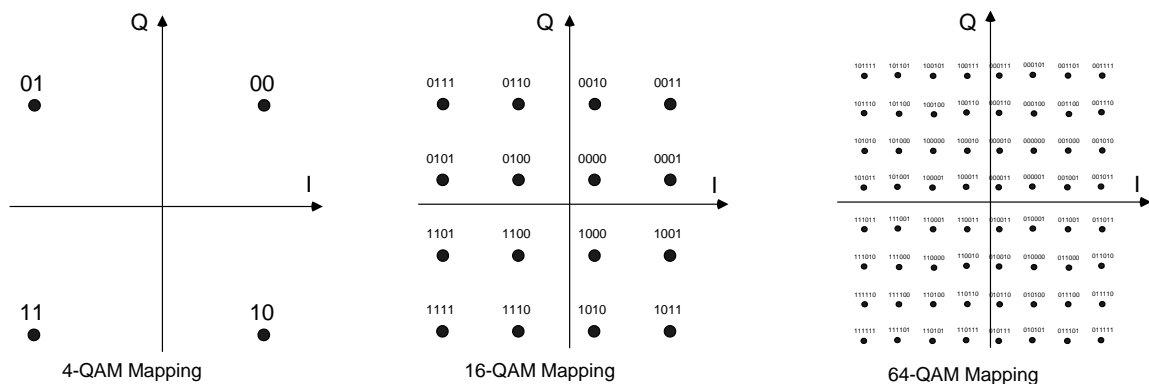
Figure 82 QAM Mappings
