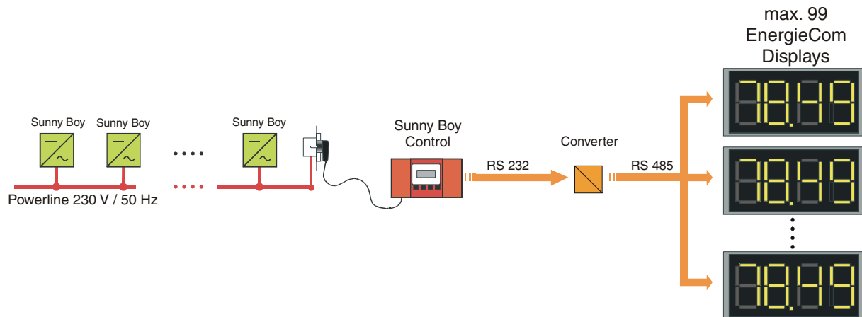
Fig. 3.13: Connection of EnergieCom displays with RS485
