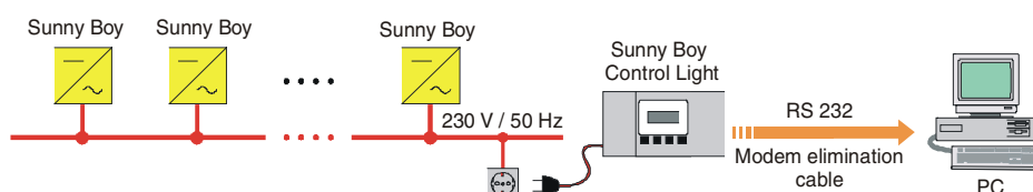
Fig. 3.2: Connection to a PC with RS232.
