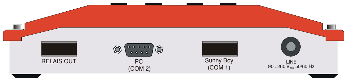
Fig. 3.1: Bottom View of the Sunny Boy Control Light with interfaces and connectors
