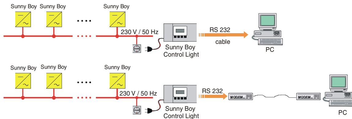
Fig. 6.1: Remote diagnosis via PC and Sunny Data Control
