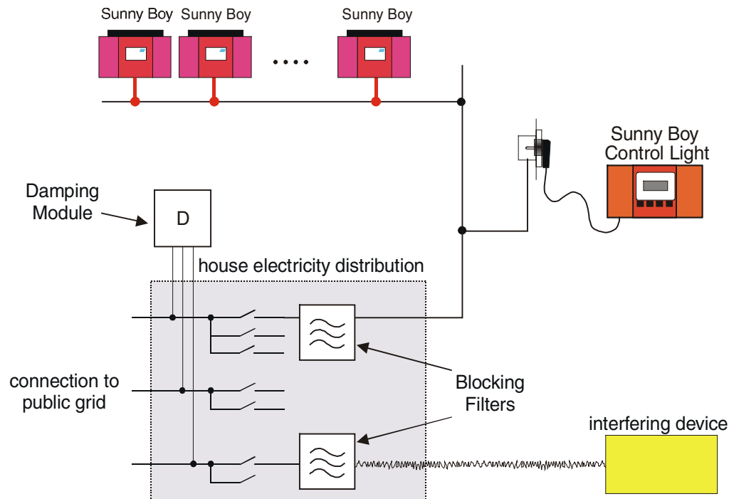
Fig.7.10: Interference suppression from several communication systems
