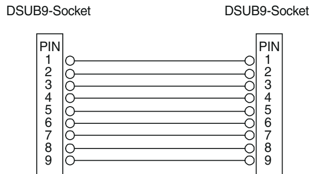
Fig. 3.9: Serial cable DSUB9<>DSUB9
