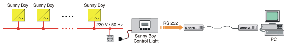
Fig. 3.8: Remote diagnosis via PC and modem
