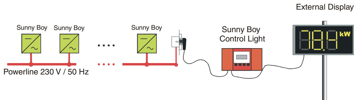
Fig. 3.11: Direct connection of an external display (DATALITE, HvG and Siebert)
