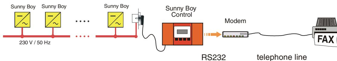
Fig. 3.10: Connecting a Modem
