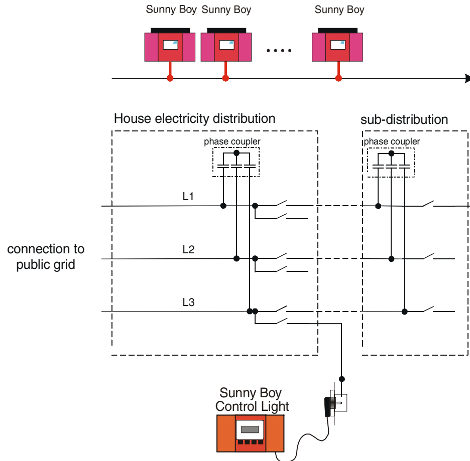
Fig. 7.8: Phase coupling for communication over different phases
