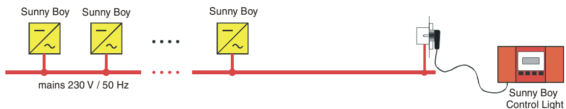
Fig. 2.6: Powerline Communication
