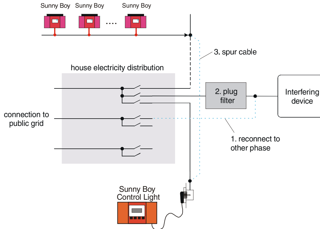
Fig.7.7: Interference suppression at strong signal damping
