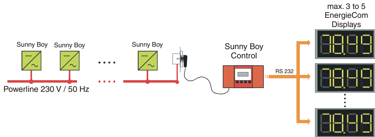
Fig. 3.12: Connection of EnergieCom displays with RS232
