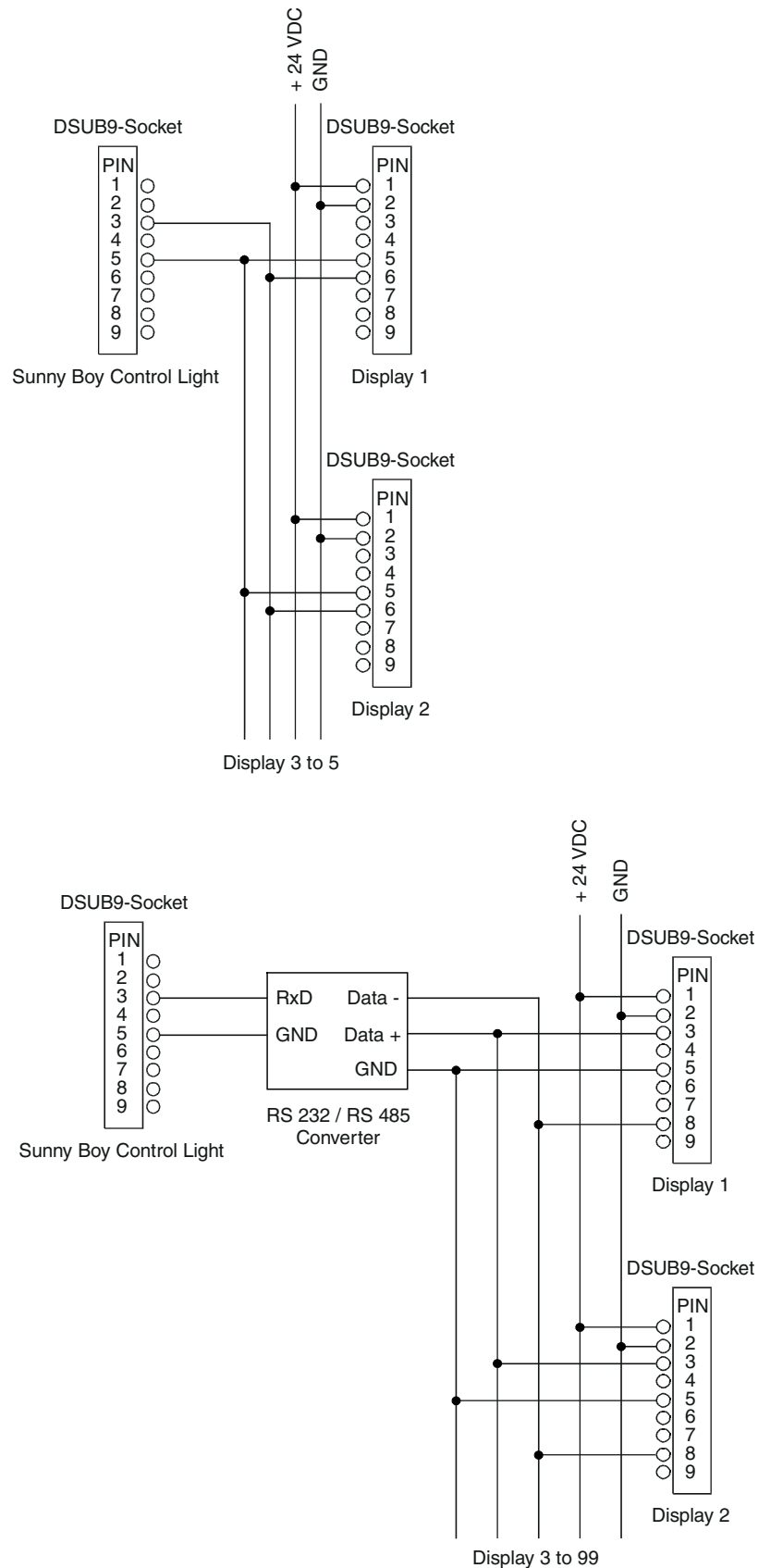
Fig. 3.14: Cabling EnergieCom displays RS232 and RS485
