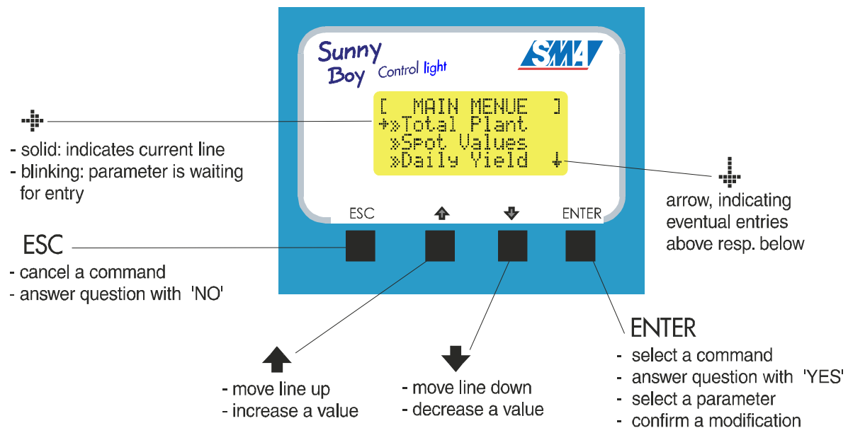
Fig. 1.1: Display and keys of the Sunny Boy Control Light
