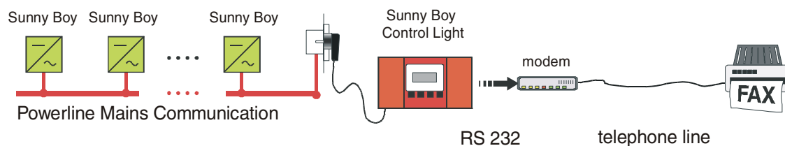
Fig. 5.36: Schematic cabling of the fax-modem connection
