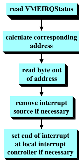
Figure 5: Handling of an Interrupt 1
