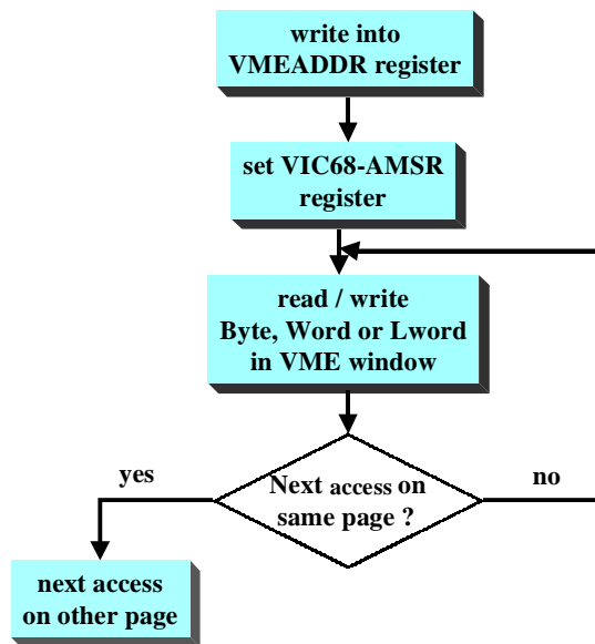
Figure 4: Steps to access the VME bus.
