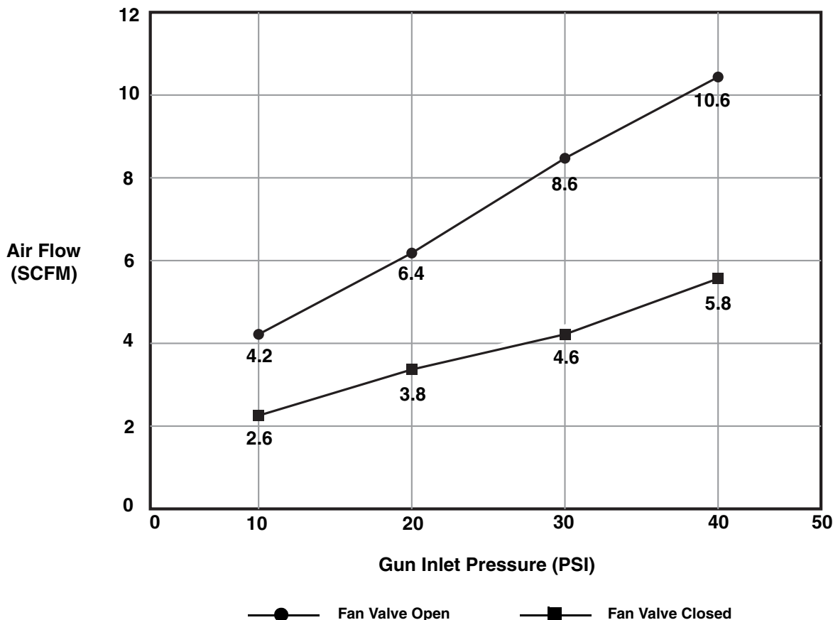
Air Flow, Standard AA Series Air Cap
