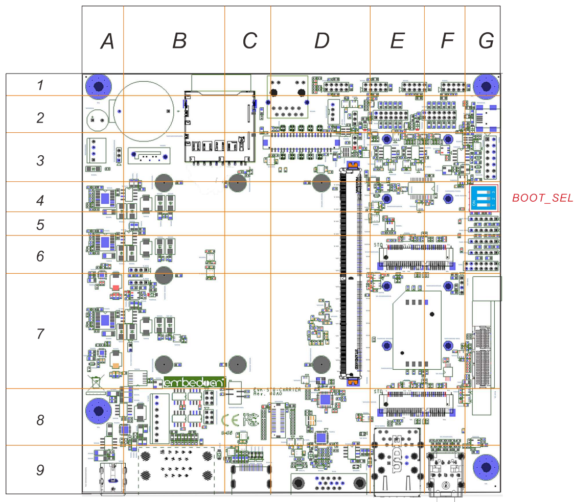
Figure 6: Switch Locations
