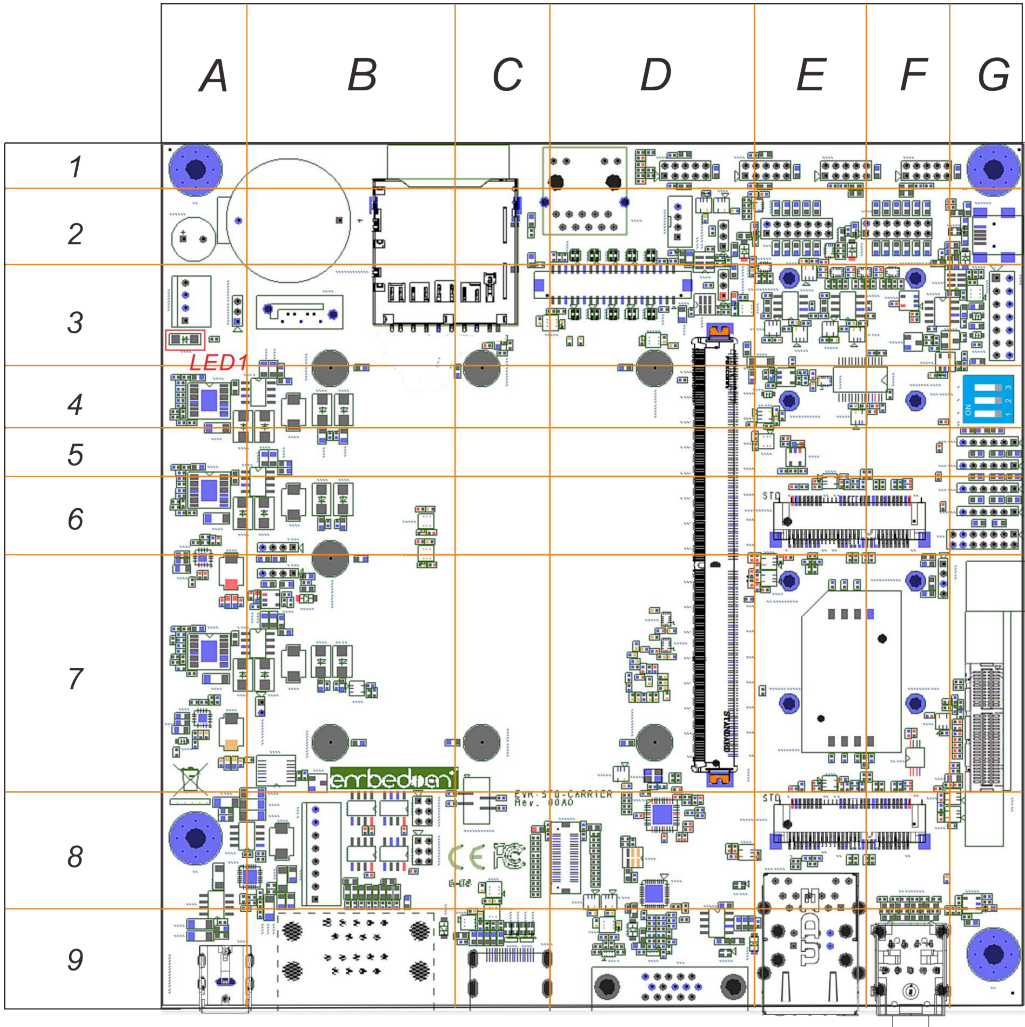
Figure 7: LED Locations
