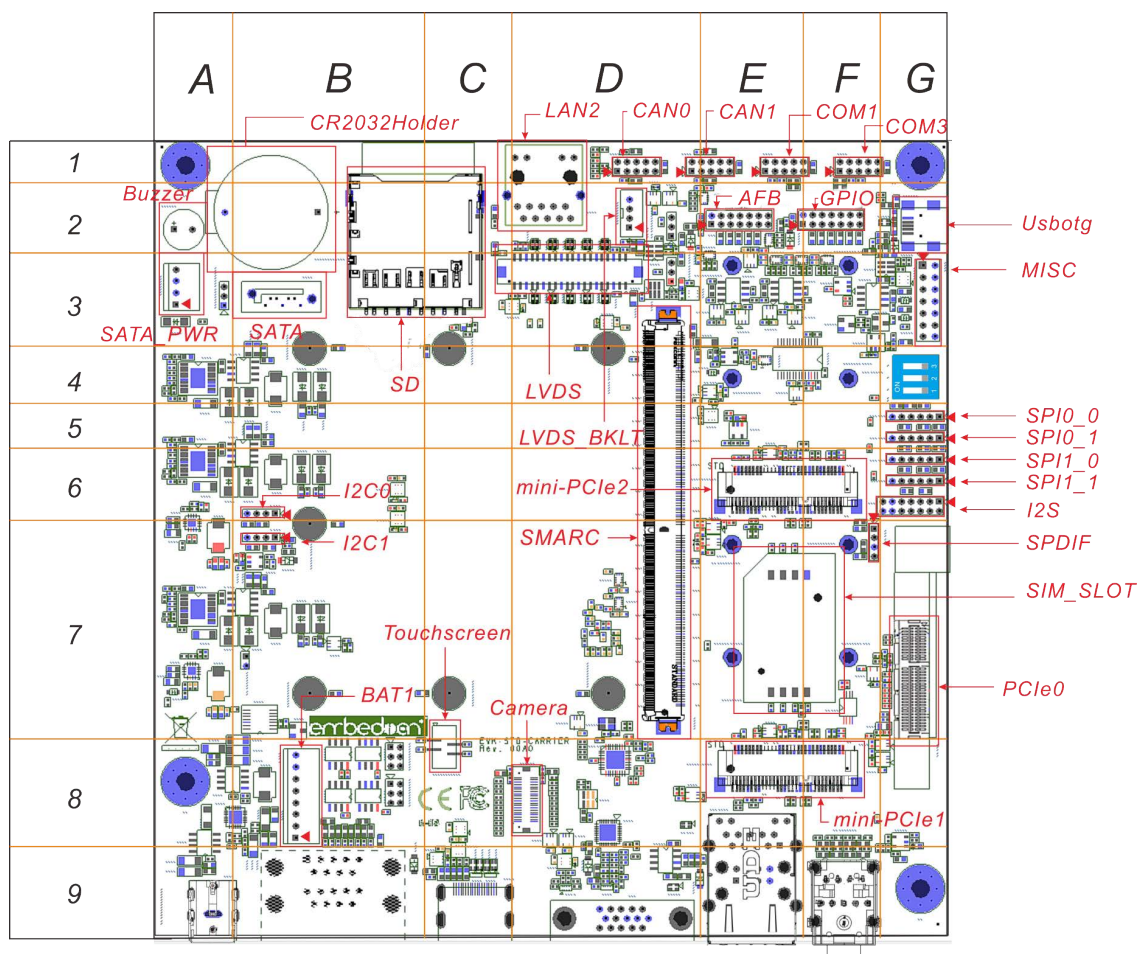
Figure 9: Internal I/O Header Locations
