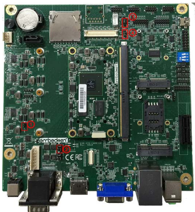
Figure 15: Check Jumper Settings
