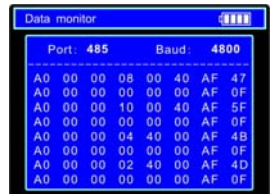
Open Line or Short Line
