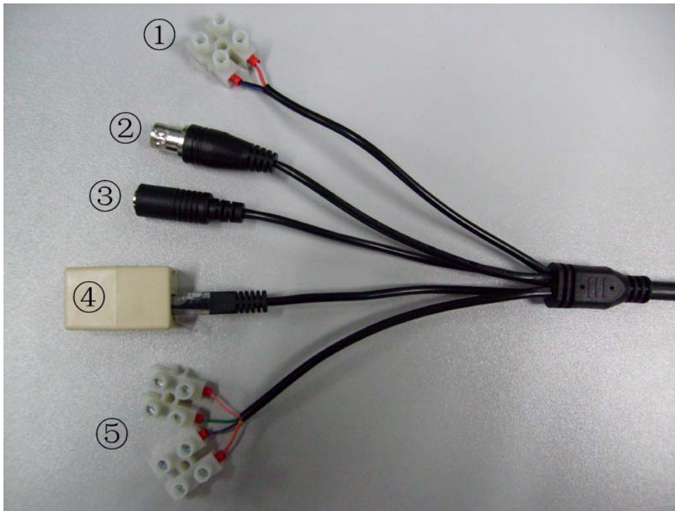
Fig. 2.1 Connection Cable
