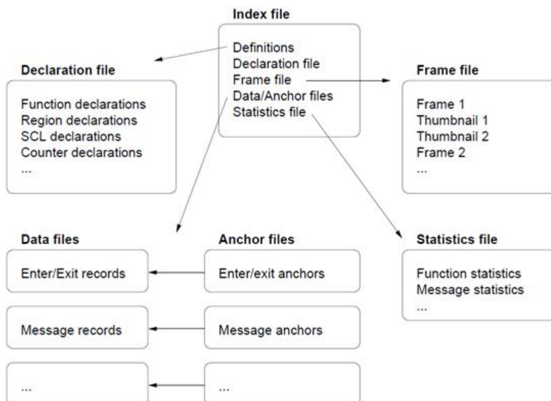
Figure 7.1 STF Components
