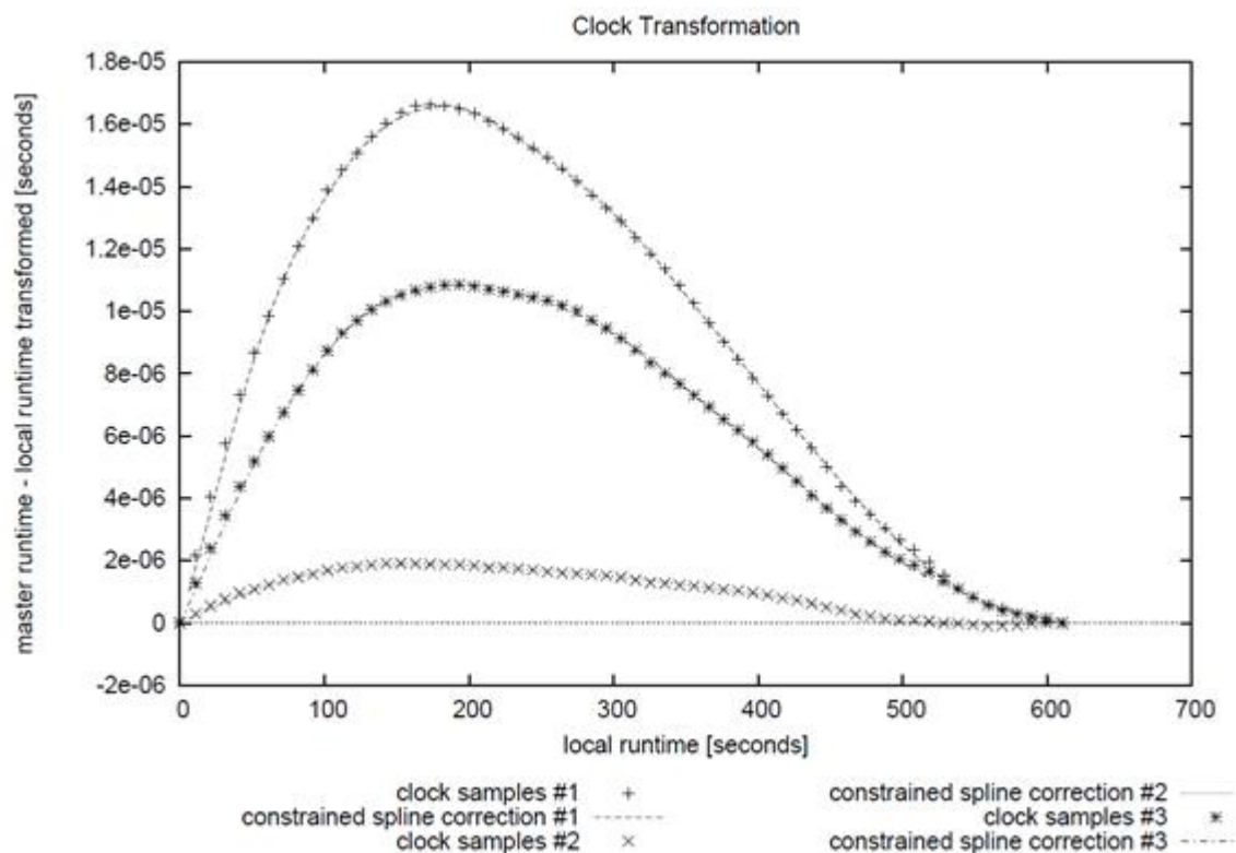
Figure 5.2 CPU Timer: clock Transformation and the Sample Points It Is Based on
