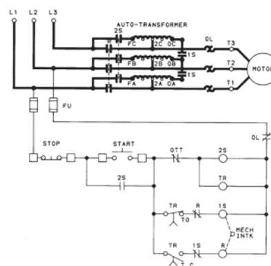
Schematic Diagram - NEMA Size 4
