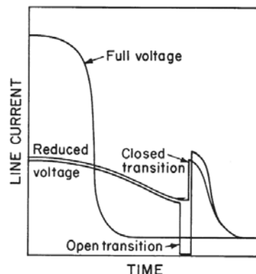
Starting Current Comparison
