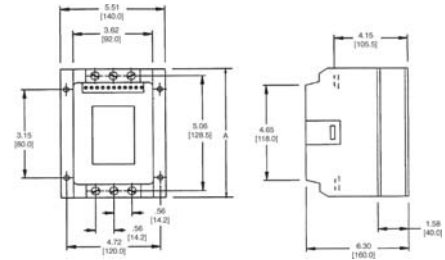
Open Starters
