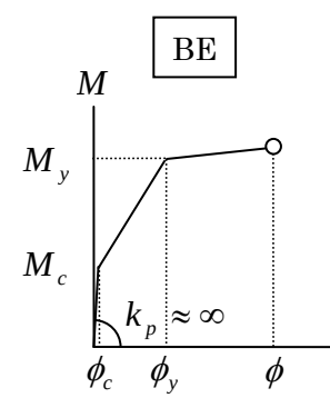
Nonlinear bending spring
