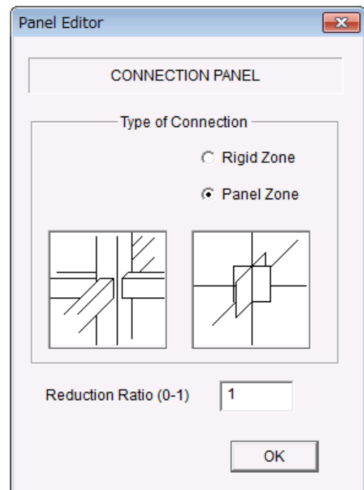
Panel Zone
