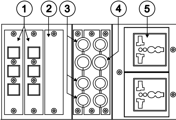
Figure 3: TBUS-6W Connecting Surface
