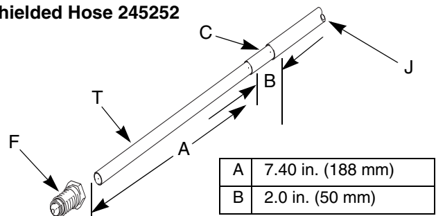
Fig. 4. Waterborne Hose Dimensions (At Gun)
