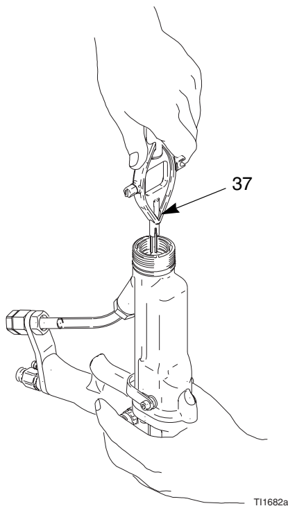
Fig. 25. Electrode Replacement
