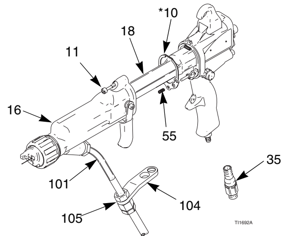
Fig. 29. Barrel Installation
