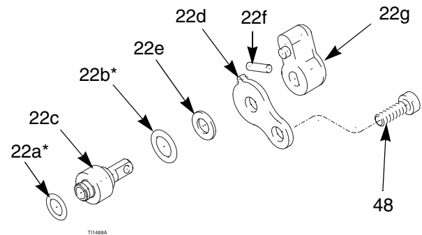
Fig. 35. ES ON/OFF Valve
