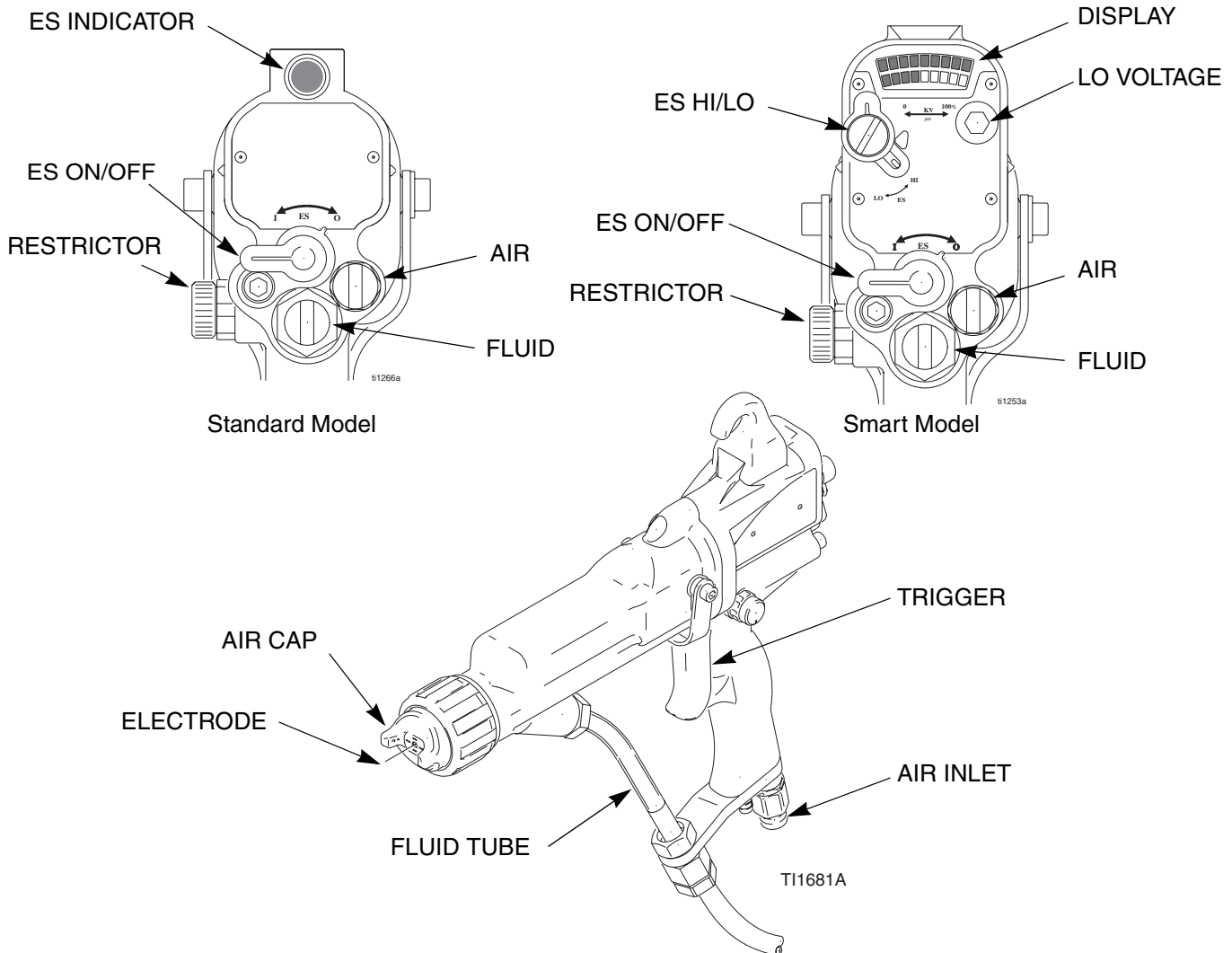
Fig. 1. Gun Overview
