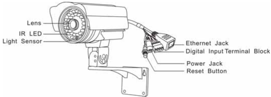
Figure 2-1: Major components of the IP camera
