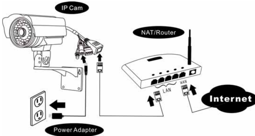
Figure 2-2: IP CAM connection diagram.
