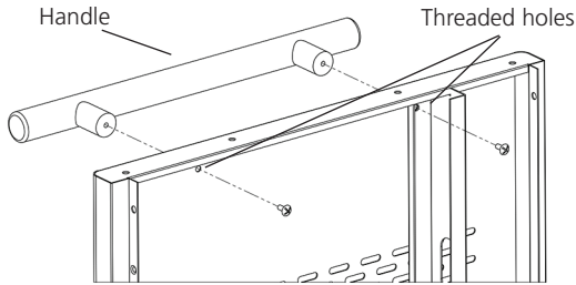
Figure 4-1. Installing handle.
