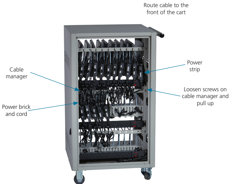
Figure 4-2. Fastening the power brick and routing the cable.
