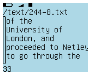
Figure 11.40.: Text Viewer
