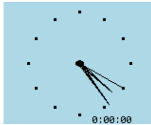
Figure 11.47.: Clock
