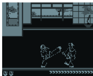
Figure 11.43.: ZXBox
