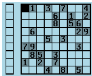
Figure 11.25.: Sudoku
