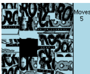
Figure 11.18.: Sliding puzzle
