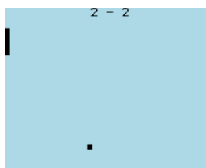
Figure 11.15.: Pong
