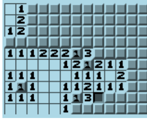
Figure 11.13.: Minesweeper plugin
