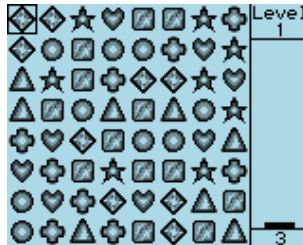
Figure 11.11.: Jewels
