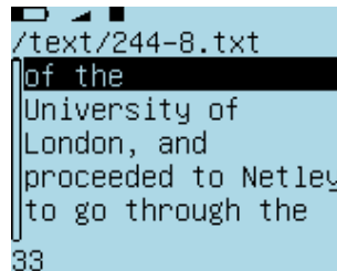
Figure 11.42.: A bookmark
