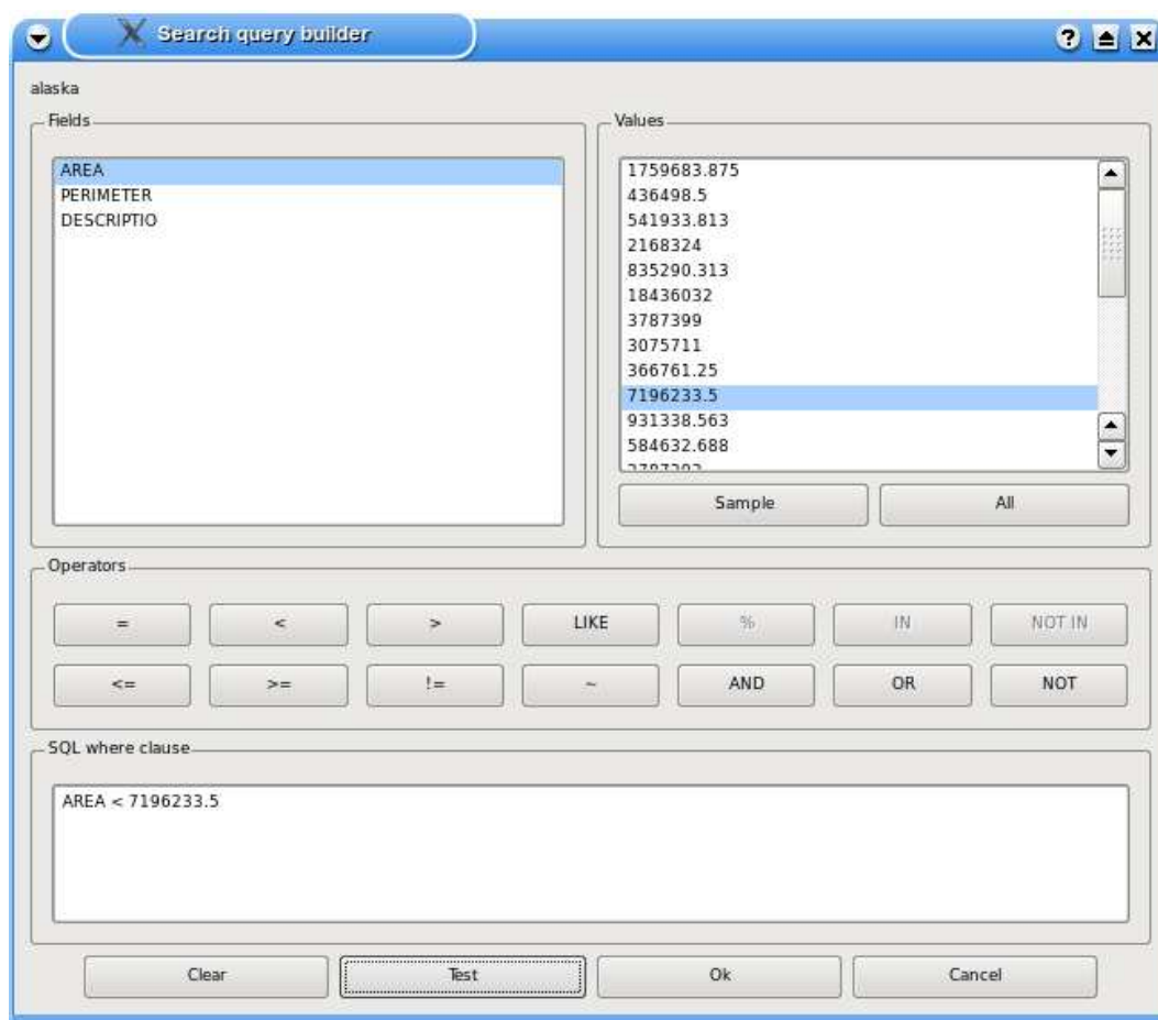
Figure 9: Query Builder
