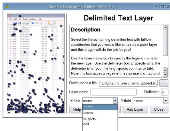
Figure 32: Fields Parsed from Text File
