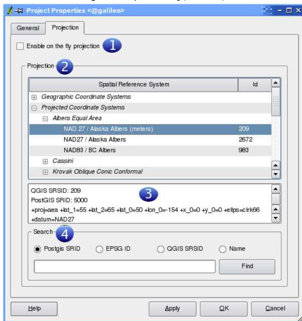
Figure 14: Projection Dialog (GNU/Linux)
