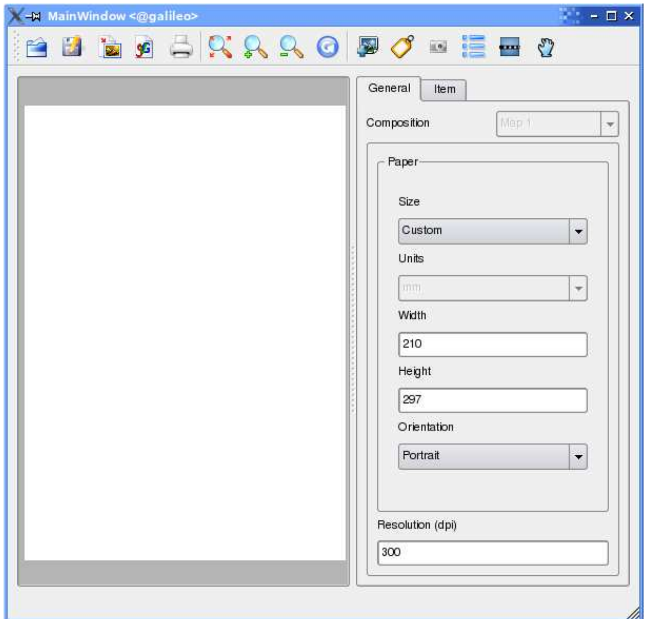
Figure 21: Map Composer
