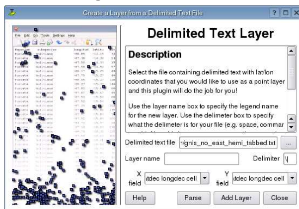
Figure 31: File Selected
