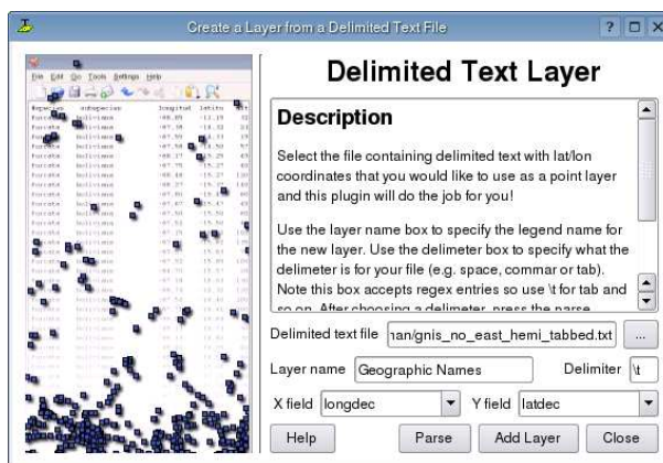
Figure 33: Selecting the X and Y Fields
