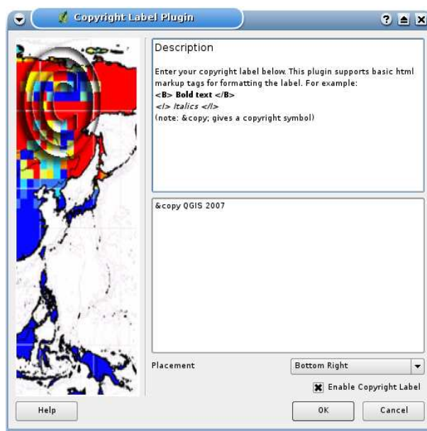
Figure 24: Copyright Plugin
