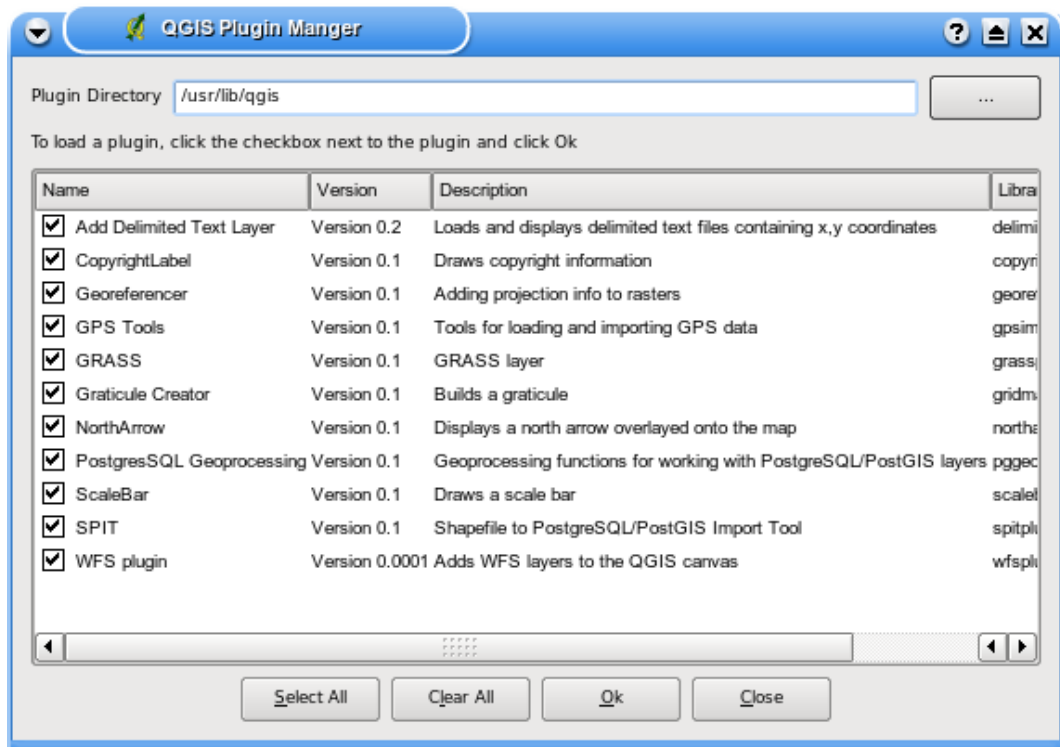
Figure 23: Plugin Manager
