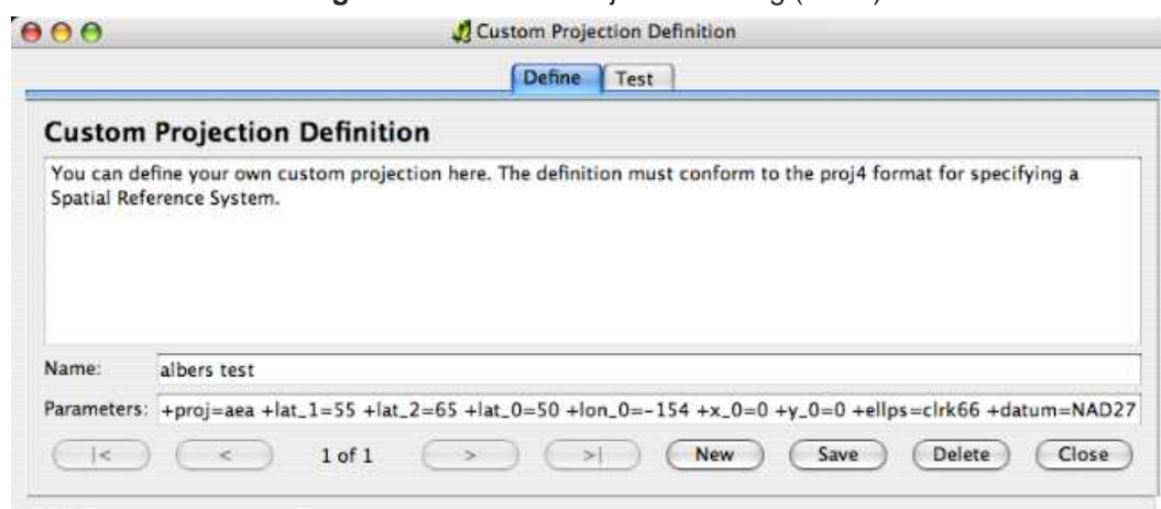
Figure 15: Custom Projection Dialog (OS X)
