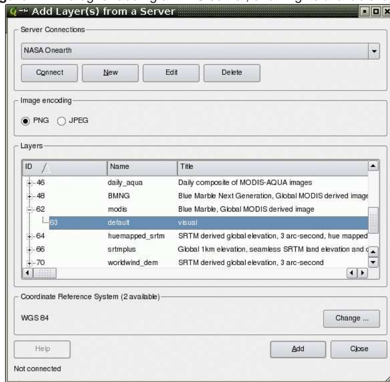
Figure 12: Dialog for adding a WMS server, showing its available layers
