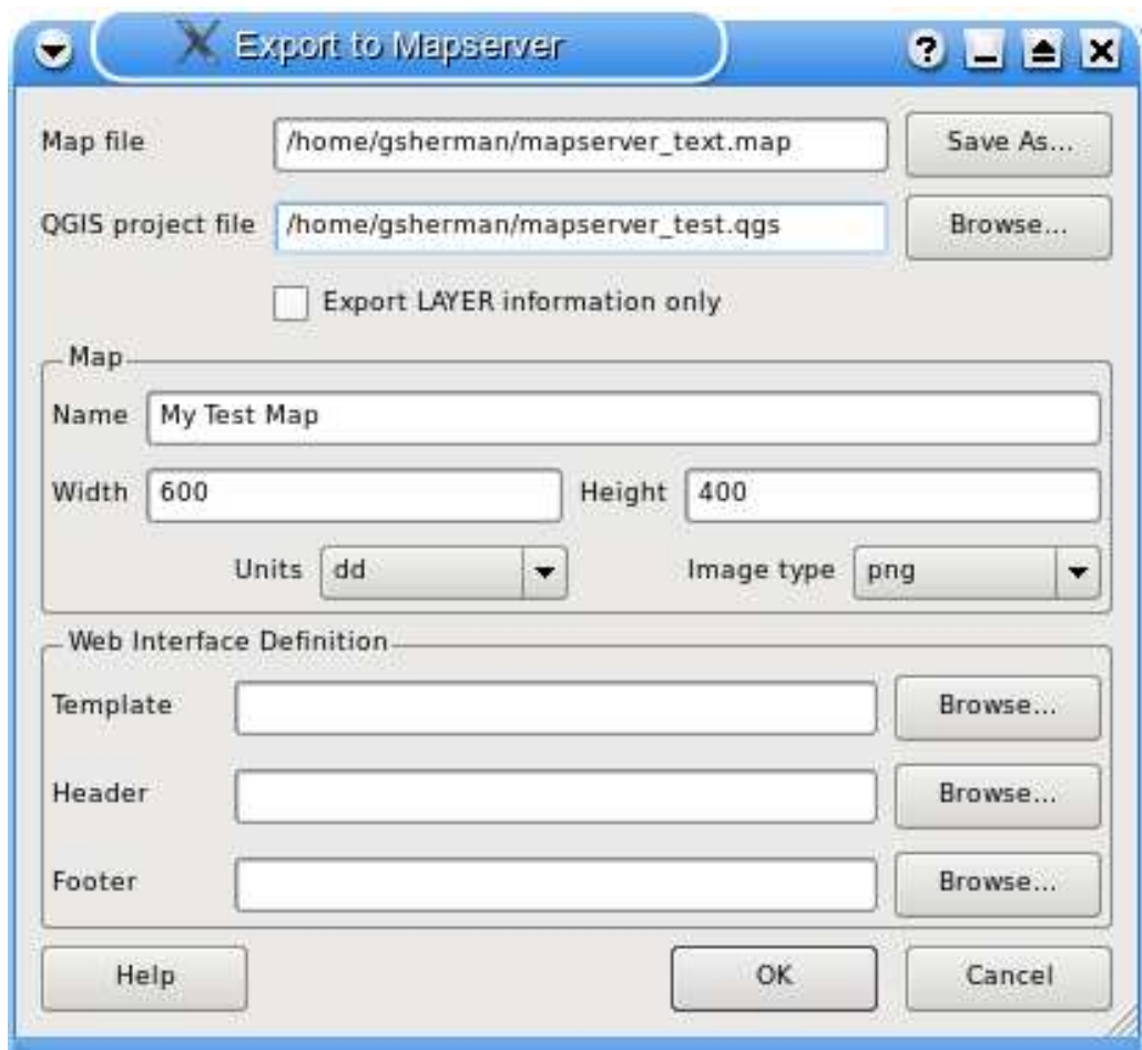
Figure 20: Export to MapServer map module in QGIS
