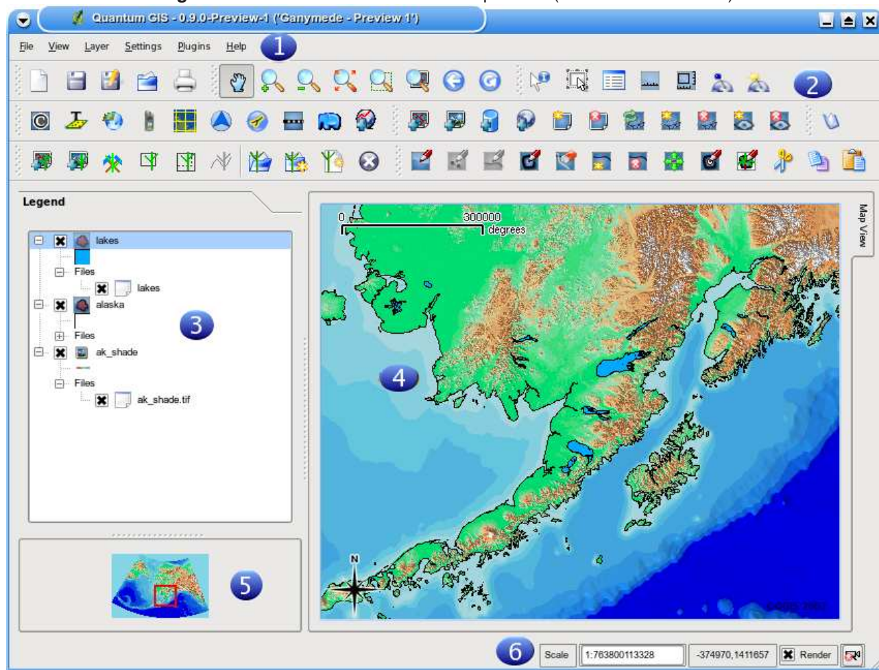
Figure 1: Main window with alaska sample data (GNU/Linux with KDE)
