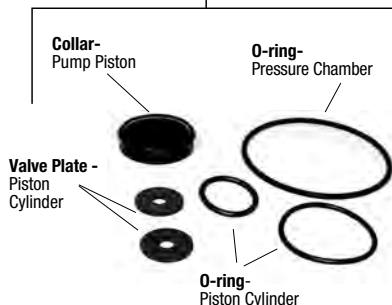
99944100471 Piston Pump Repair Kit
