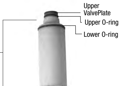
99944100474 Piston Cylinder Assembly
