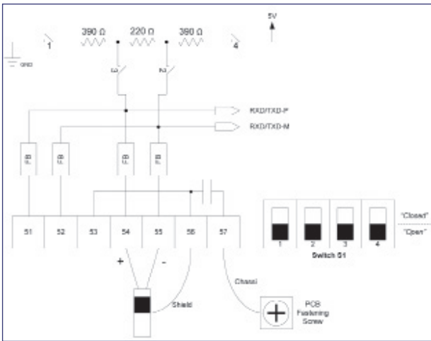
Figure 4: Signal Wiring Diagram
