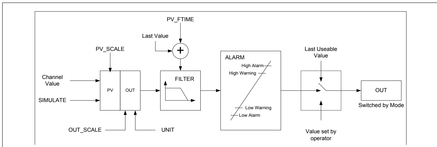
Figure 6: Analog Input Function Block Structure
